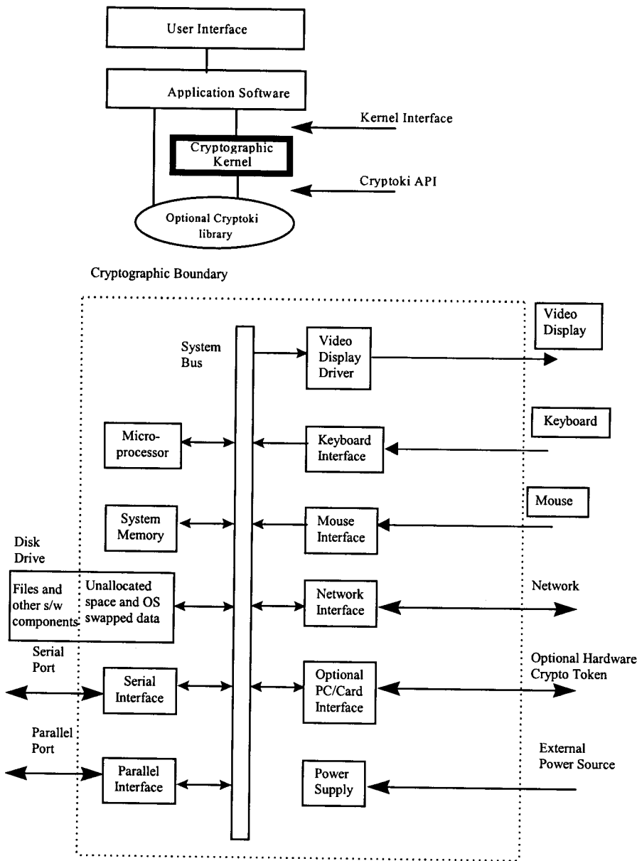
Figure 1 Cryptographic module block diagram for hardware (bottom) and software (top)
