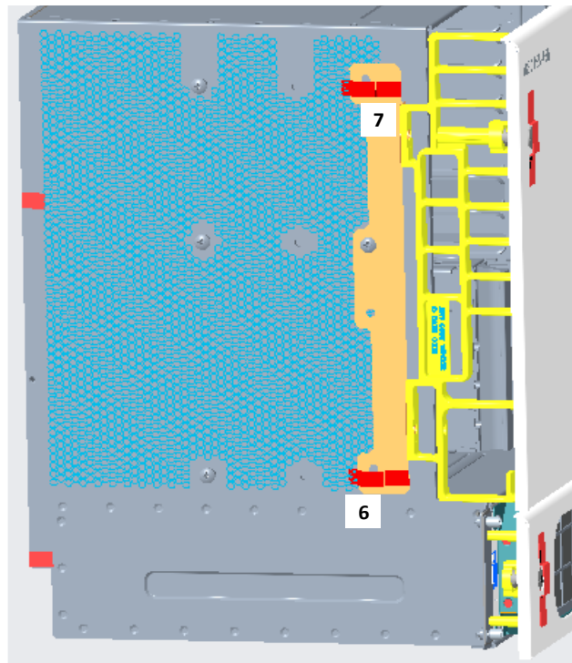
Figure 22 - Left of Nokia 1830 PSS-16II shelf
