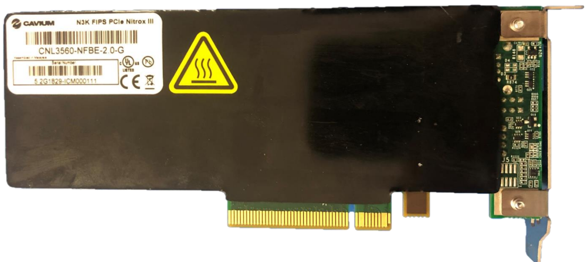
Figure 3 – Top View and Bottom View of Cryptographic Module ( HW-2.0)
