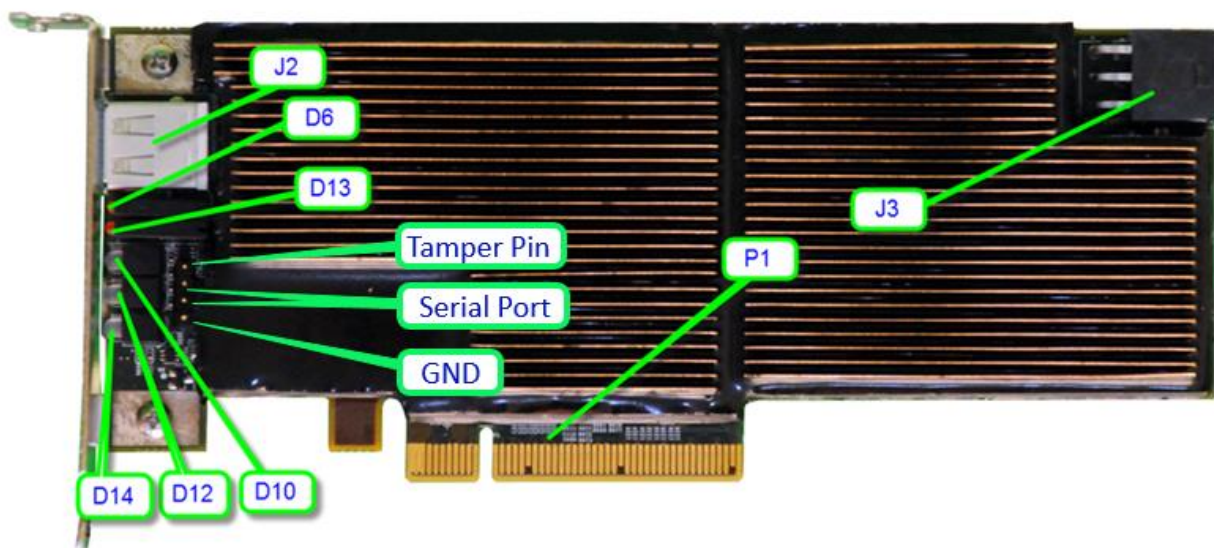
Figure 2: Photo of CryptoBind HSM and CryptoBind DSS embedded with NITROX III CNN35XX-NFBE HSM family for Securely storing and using Cryptographic Keys and Master Key
