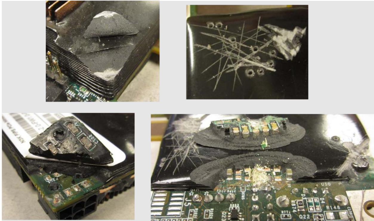
Figure 5 – Cryptographic Module Showing Tamper Evidence
