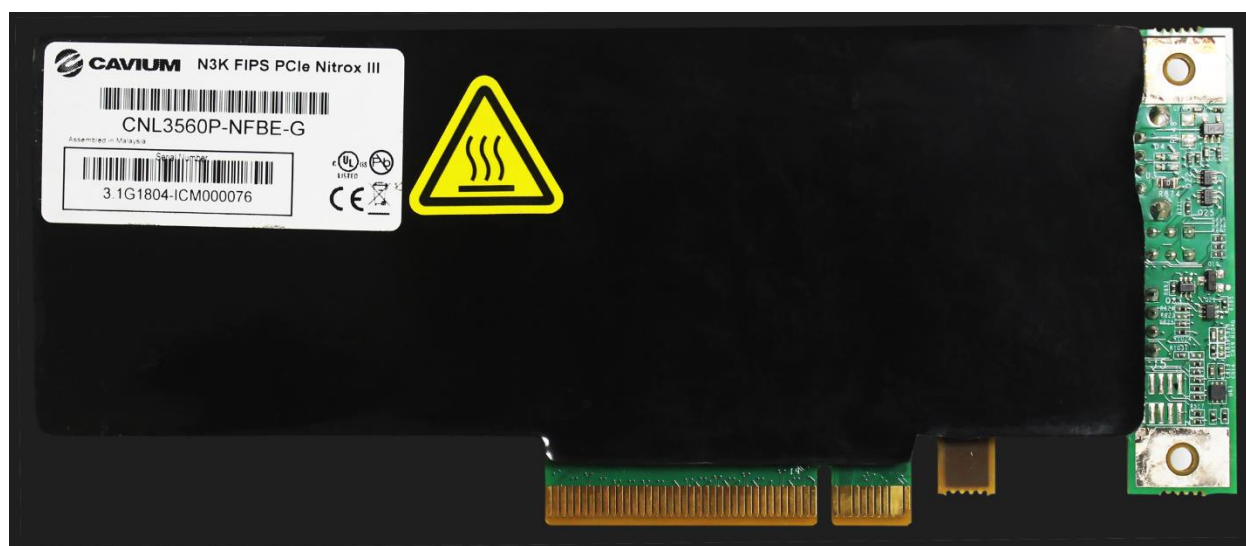
Figure 1 – Top View and Bottom View of Cryptographic Module (HW-1.0)
