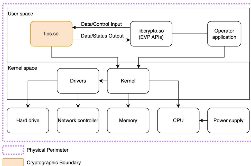
Figure 1: Block Diagram
