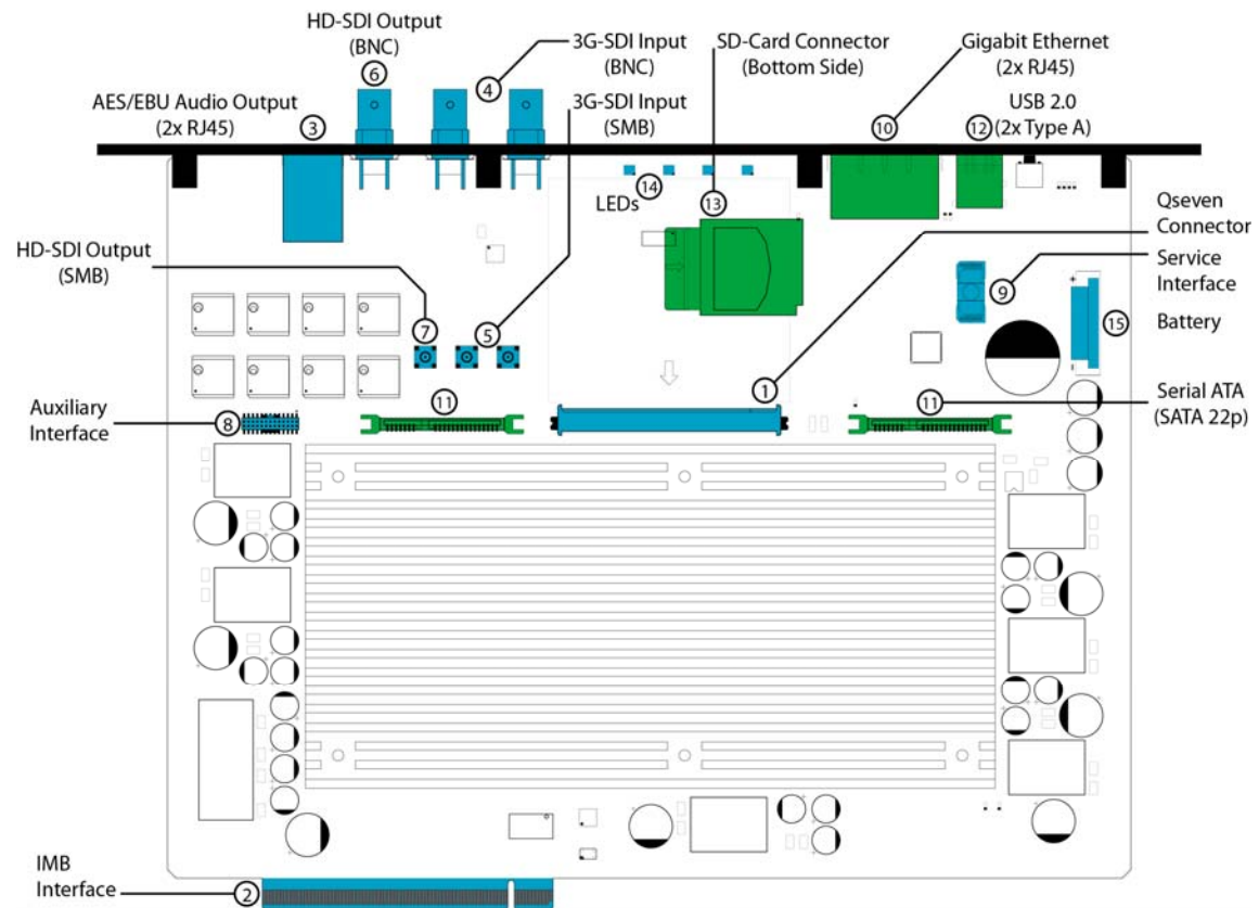
Figure 4 – Physical connectors
