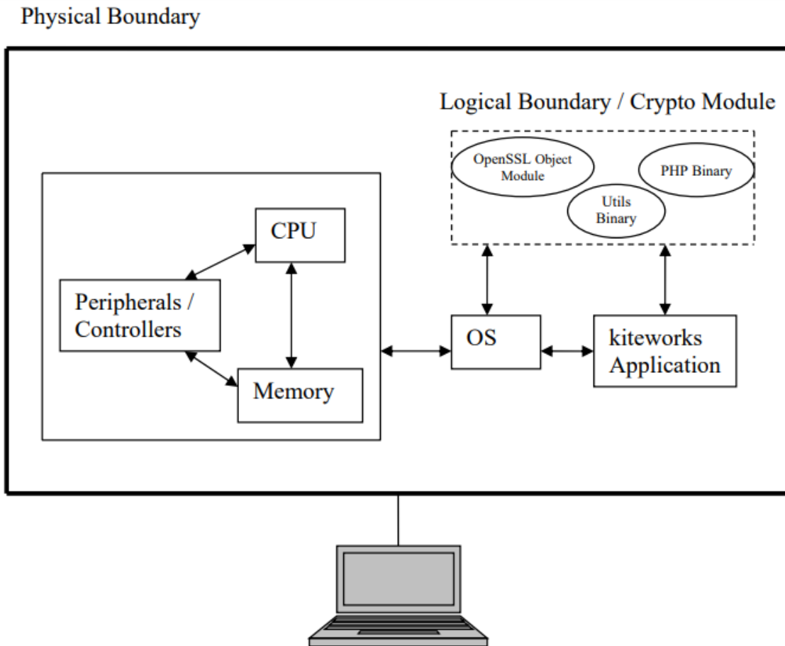
Figure 1 - Block Diagram of the Cryptographic Module
