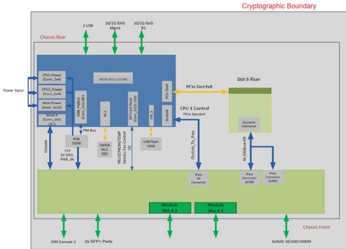
Figure 3: Block Diagram of the Trellix Intrusion Prevention System Sensor NS7500
