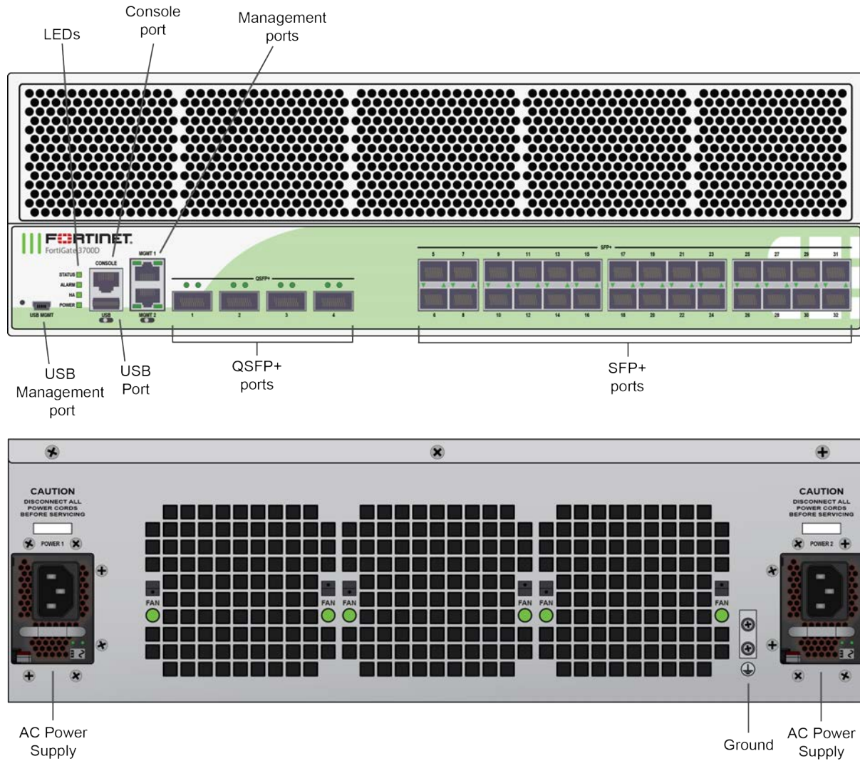
Figure 9 - FortiGate-3700D Front and Rear Panels
