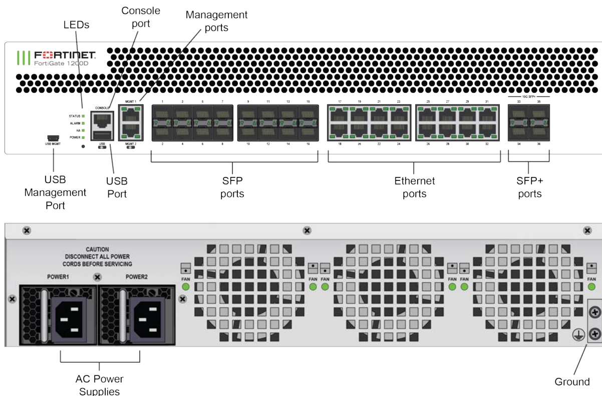
Figure 6 - FortiGate-1200D Front and Rear Panels
