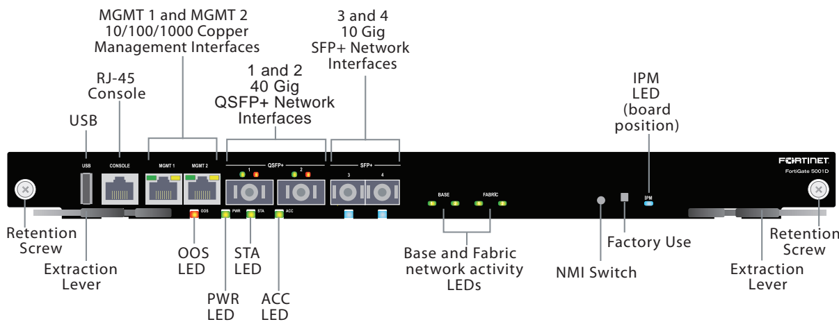
Figure 1 - FortiGate-5001D Front Panel
