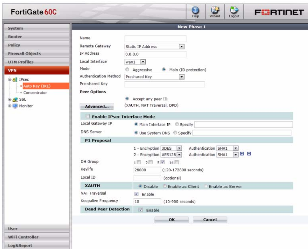
Figure 2: The FortiWiFi web-based manager
