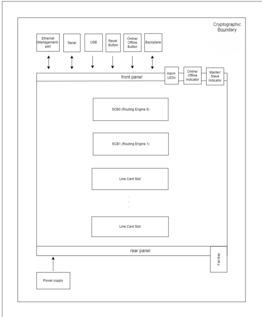
Figure 2: Block Diagram
