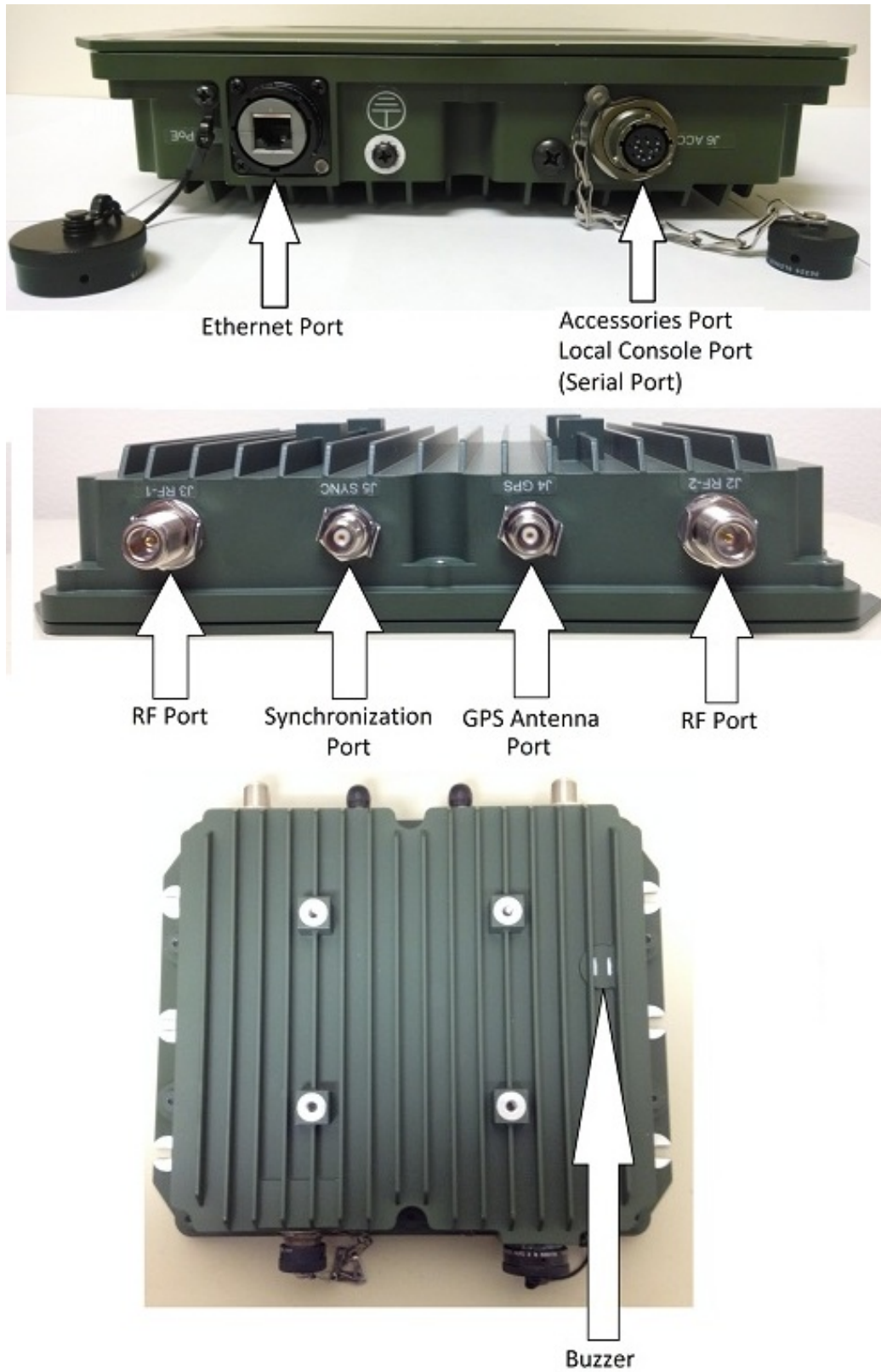
Figure 2 – Location of Physical Interfaces – 12069-3010-xx
