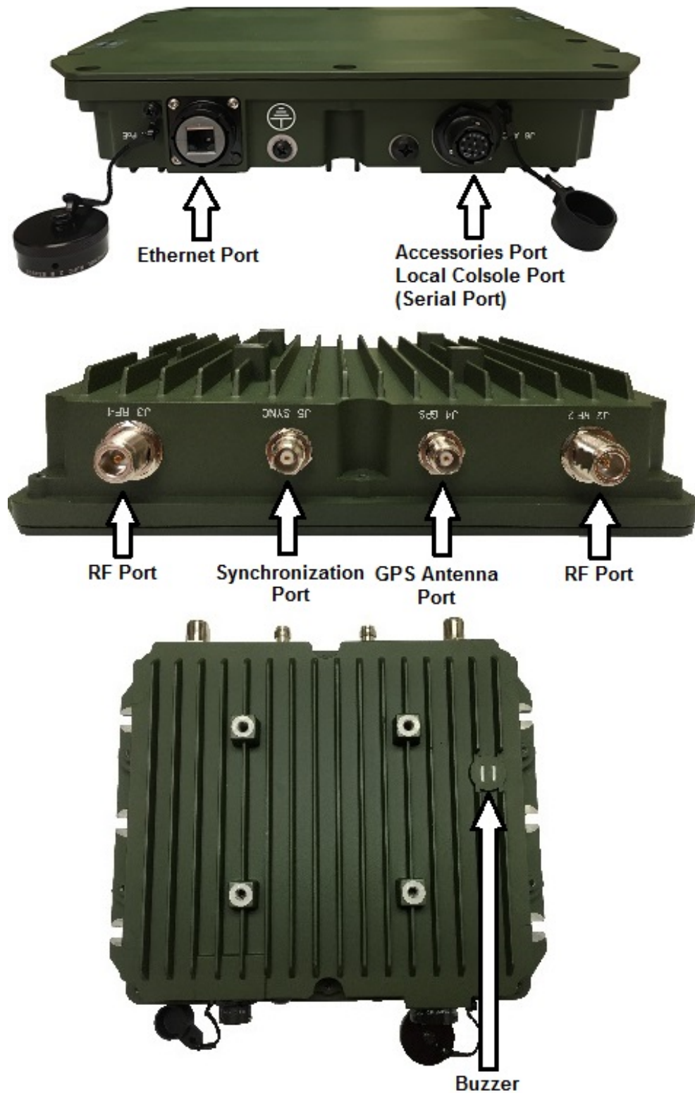
Figure 3 – Location of Physical Interfaces – 12069-3035-xx
