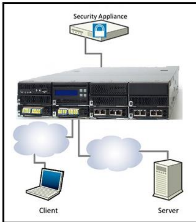
Figure 2-2 Passive-Inline Configuration
