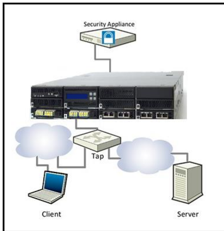
Figure 2-3 Passive-Tap Configuration
