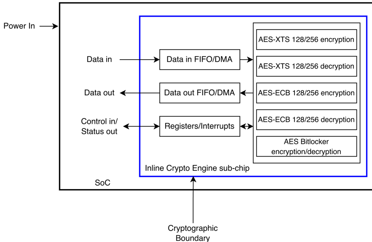
Figure 1: Cryptographic boundary and physical perimeter
