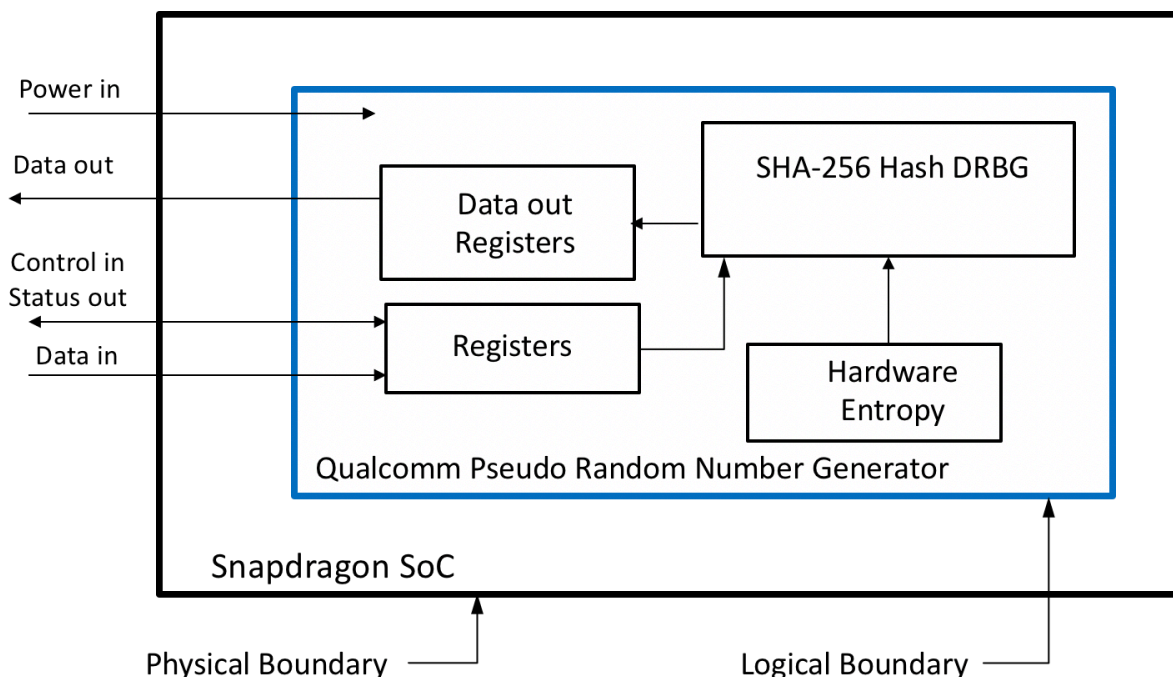
Figure 1: Cryptographic Boundary
