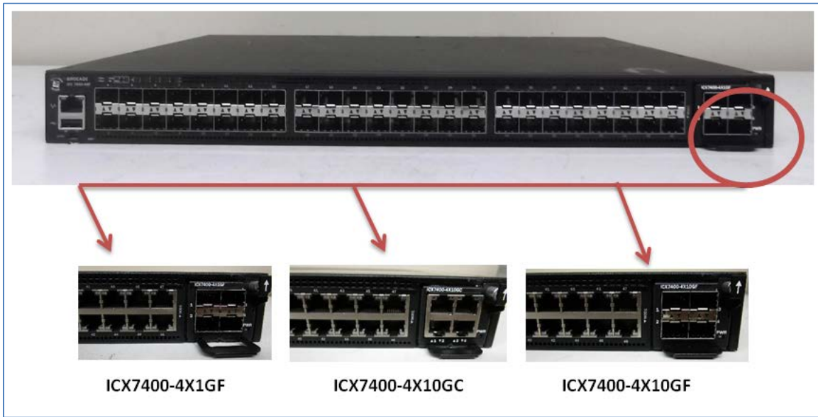
Figure 8 - Front/top side of the module ICX7450-48F with ICX7400-4X1GF, ICX7400-4X10GC and ICX7400-4X10GF
