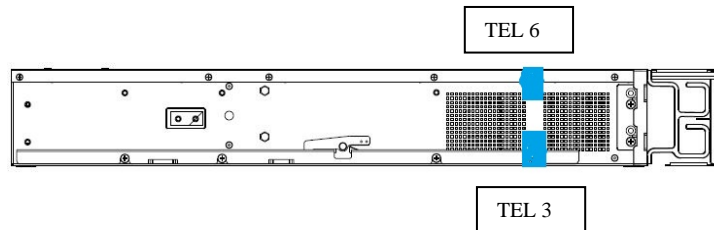
Figure 29 Cisco ASA 5585 Security Appliance with Tamper Evident Label Placement (Left Face)
