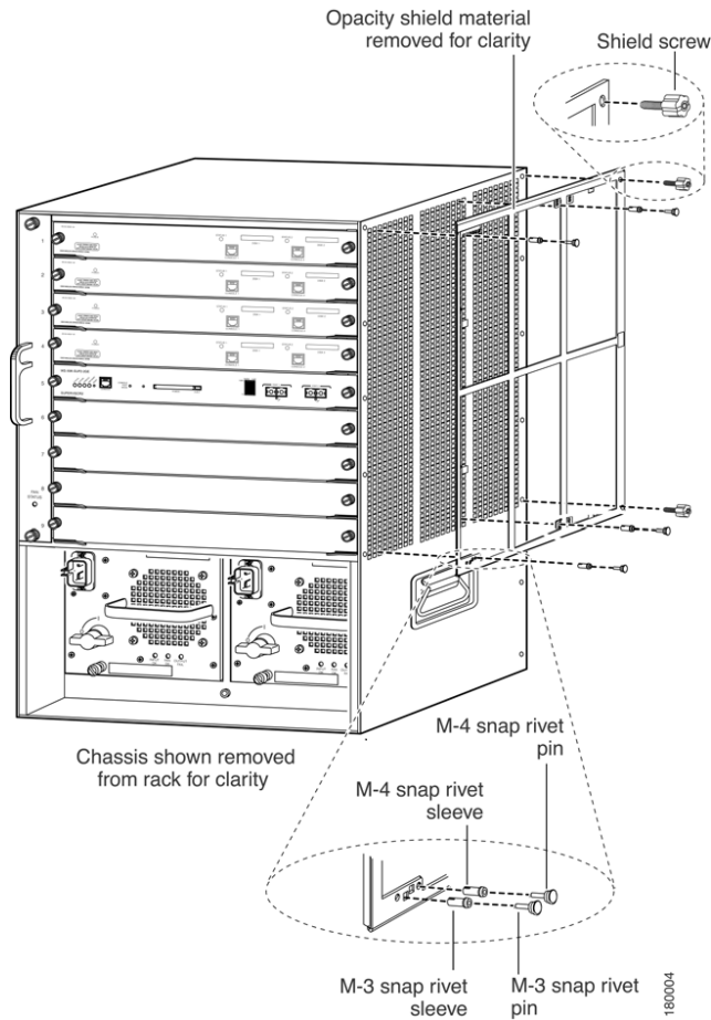
Figure 2: Cisco Catalyst 6509-E Opacity Shield Installation
