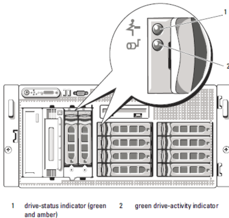
Figure 4 – Hard Drive Indicators
