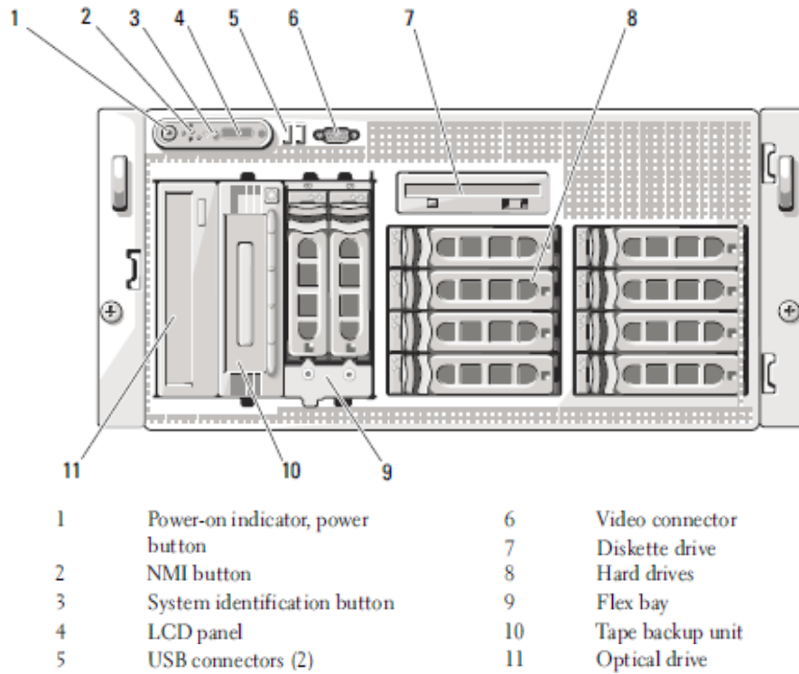
Figure 3 – Front Panel Features and Indicators
