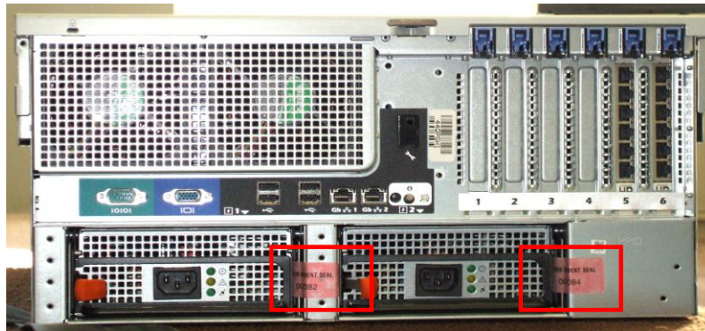
Figure 8 – Tamper-Evident Seal Application Positions (Power Supplies)
