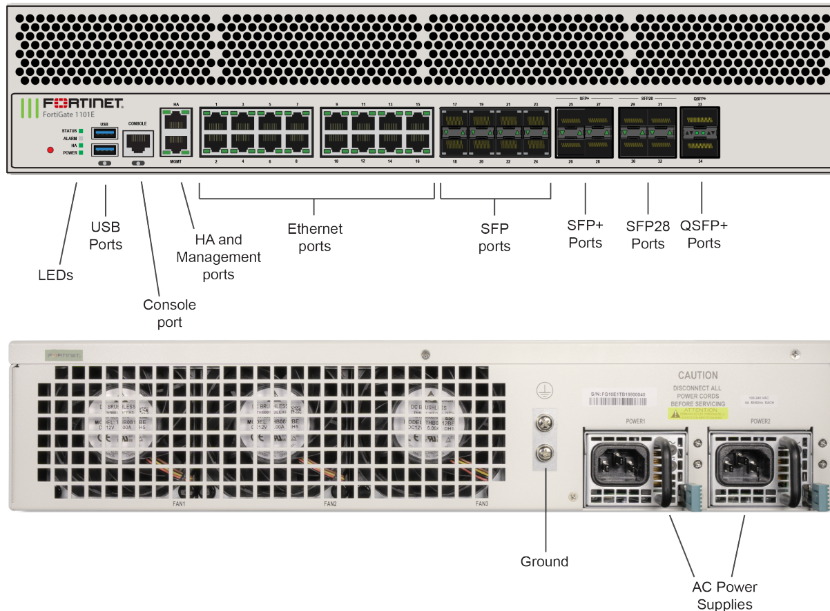
Figure 1 - FortiGate-1101E Front and Rear Panels
