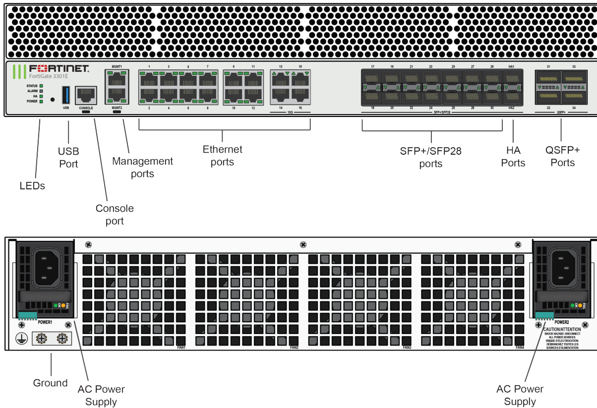
Figure 5 - FortiGate-3301E Front and Rear Panels
