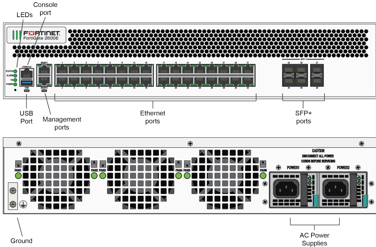
Figure 4 - FortiGate-2500E Front and Rear Panels
