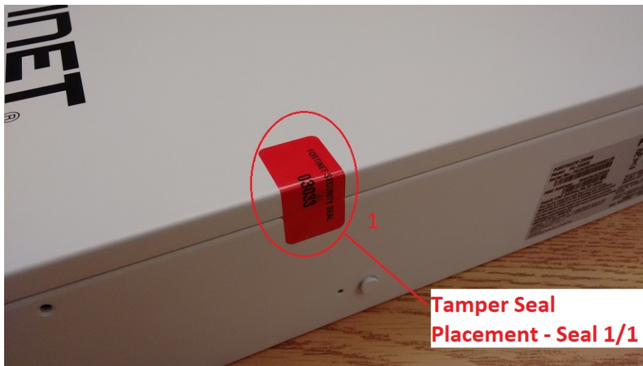
Figure 6 - FortiGate-2000E and 2500E external enclosure seal, top, right side
