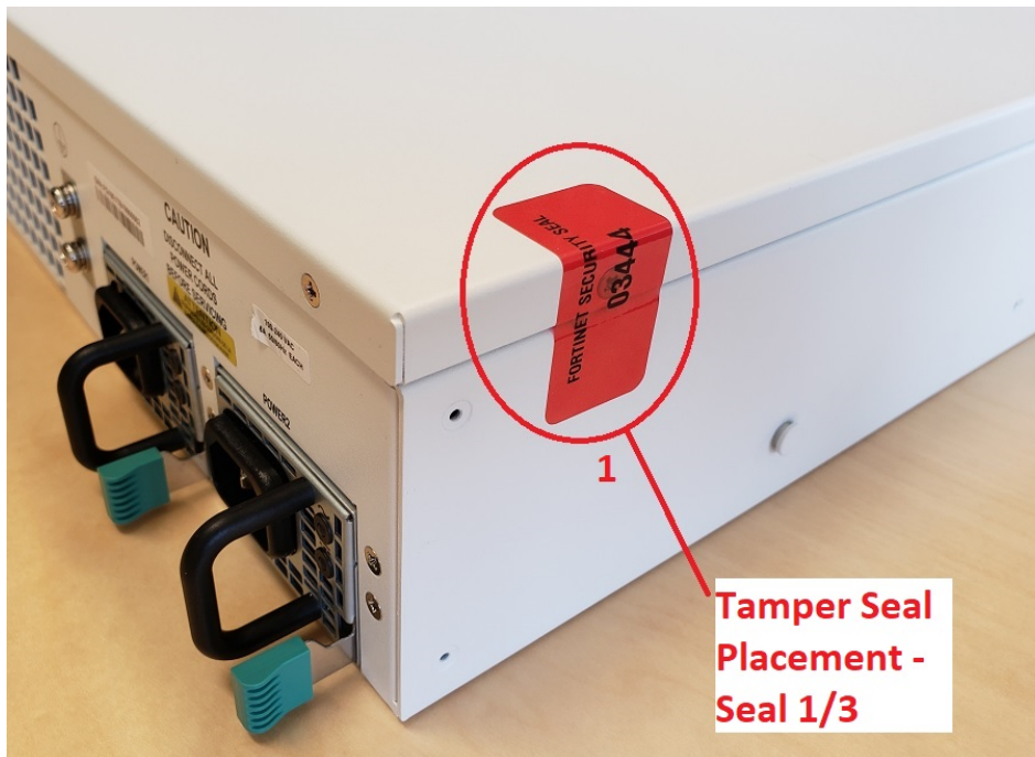
Figure 7 - FortiGate-1101E external enclosure seal, top, left side
