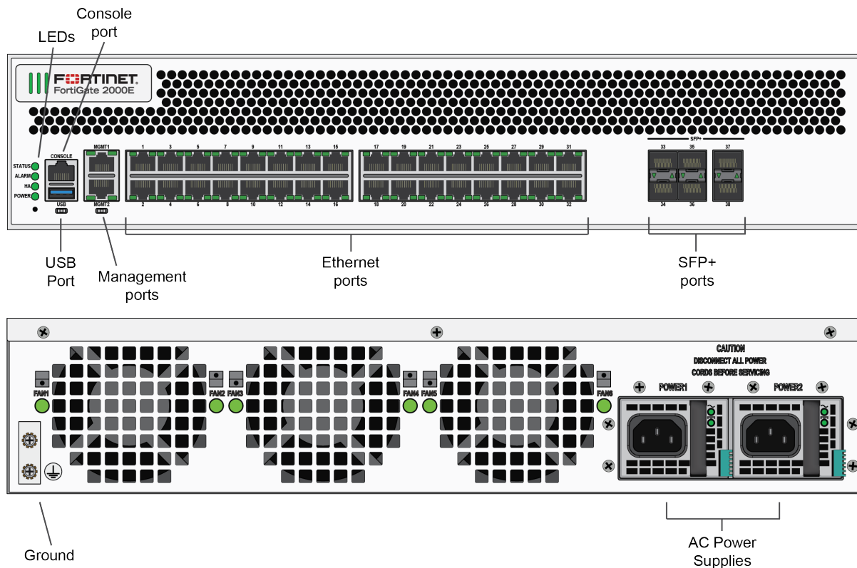
Figure 2 - FortiGate-2000E Front and Rear Panels
