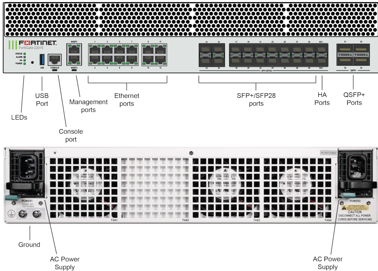
Figure 3 - FortiGate-2201E Front and Rear Panels
