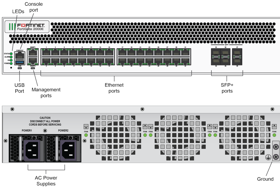
Figure 1 - FortiGate-2000E Front and Rear Panels
