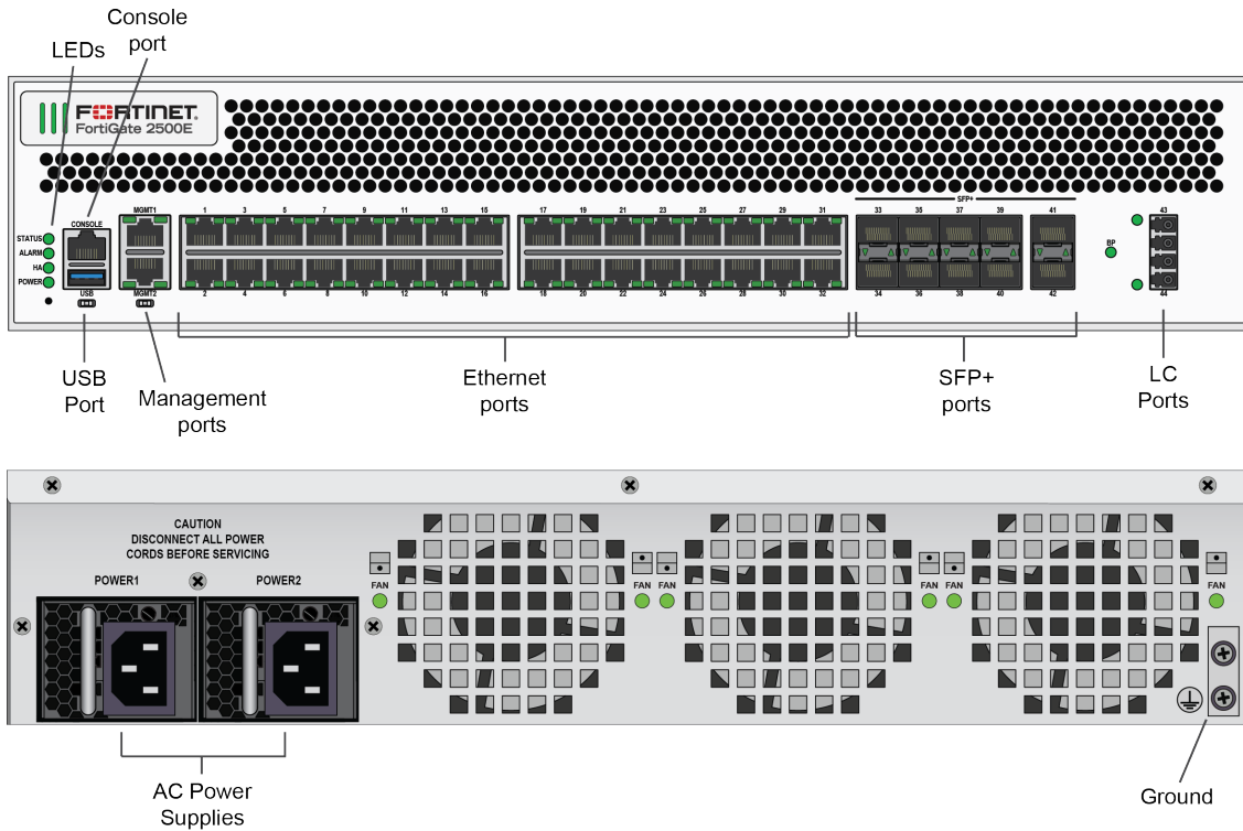
Figure 2 - FortiGate-2500E Front and Rear Panels
