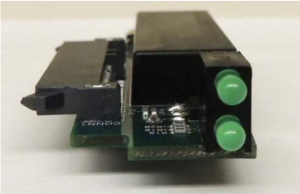
Figure 5 – KDH3000-CM – Back side view demonstrating the LEDs.
