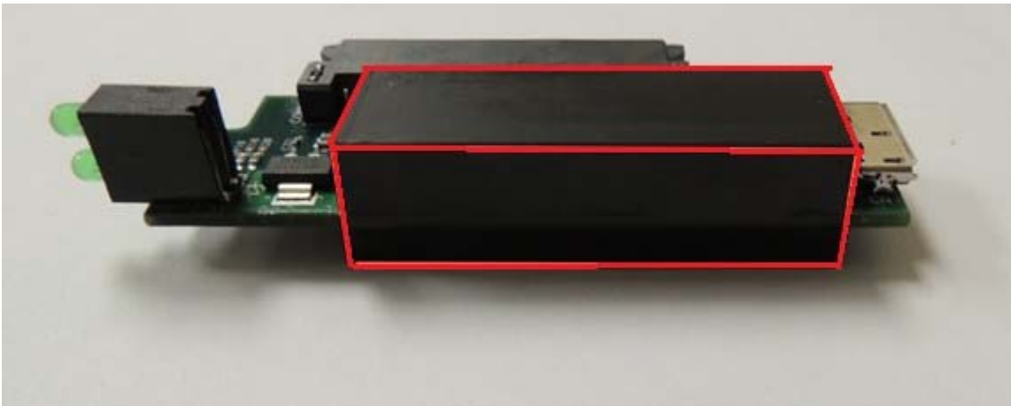
Figure 2 – KDH3000-CM – Bottom side view. The cryptographic boundary is defined by the area that the epoxy potting covers, which is outlined in red.
