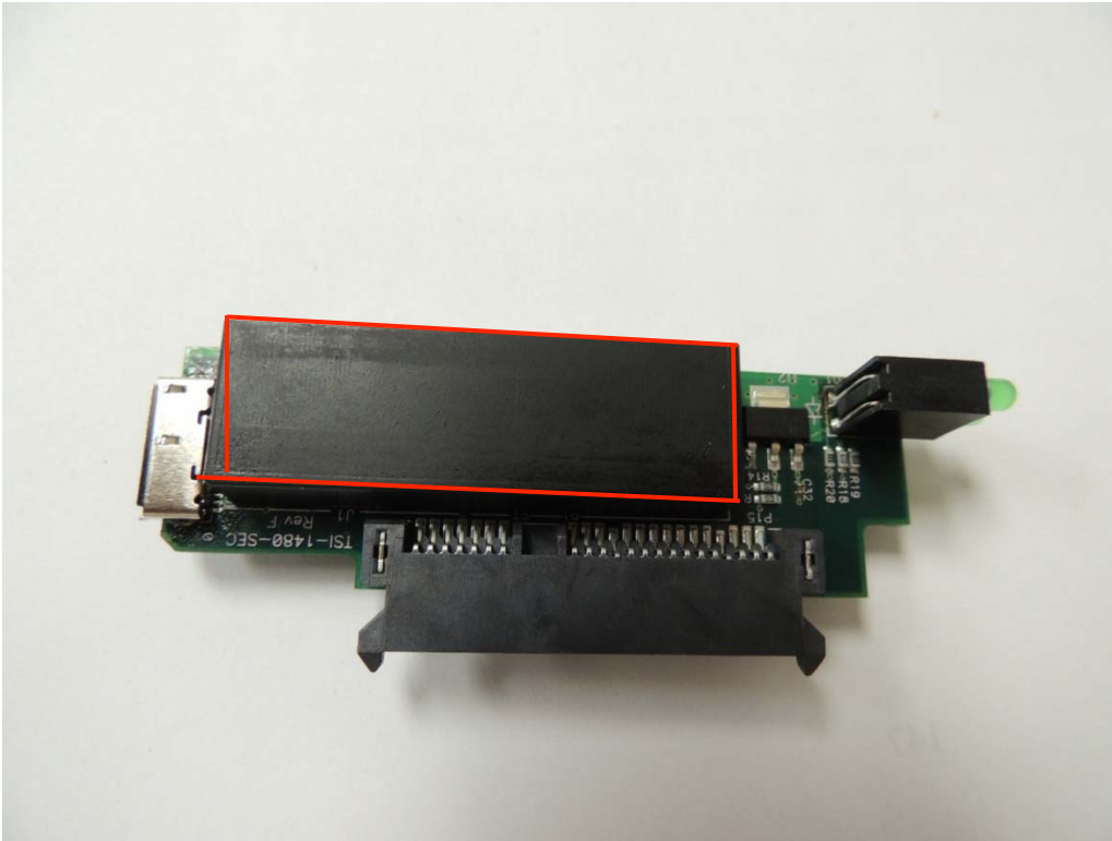
Figure 1 – KDH3000-CM – Top side view. The cryptographic boundary is defined by the area that the epoxy potting covers, which is highlighted in red.
