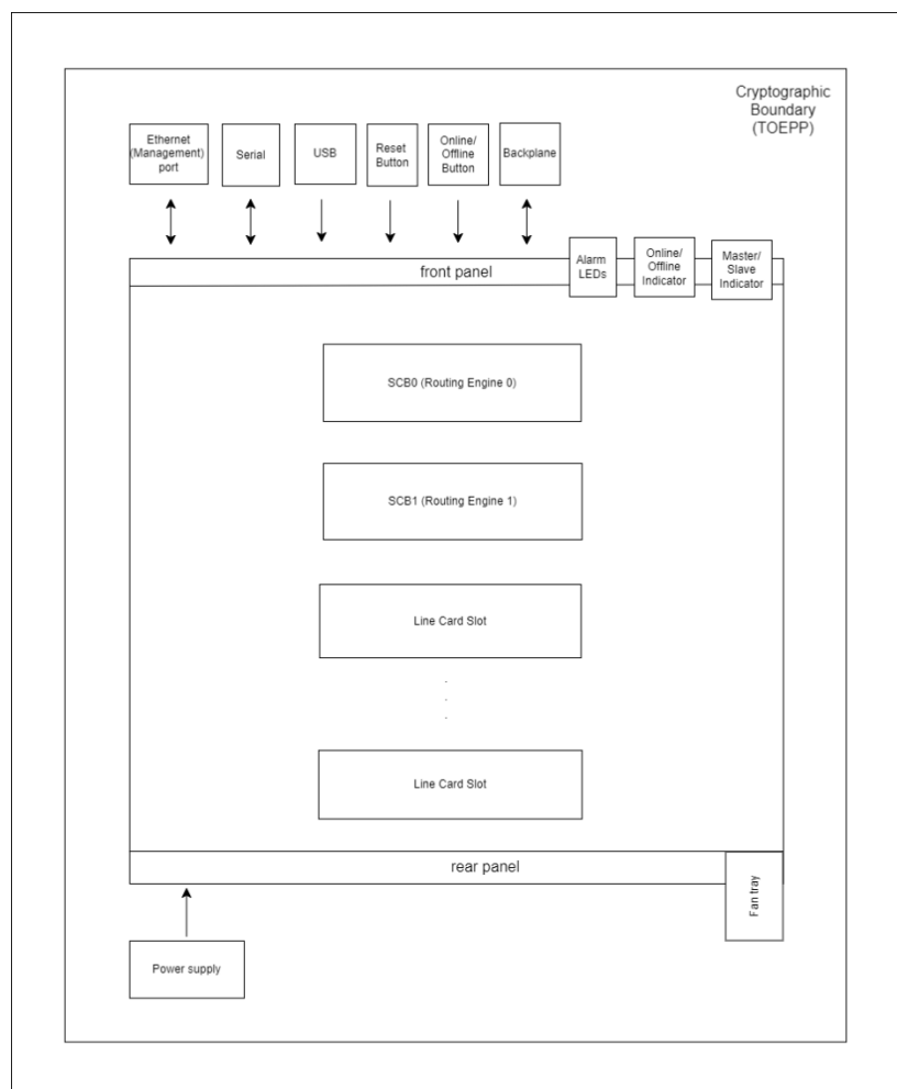
Figure 2: Block Diagram
