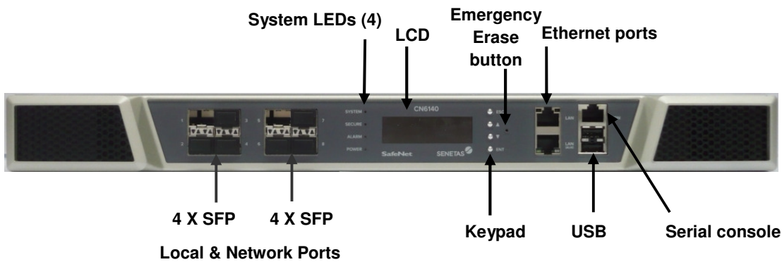
Figure 8 - Front View of the CN6140 [Y] Encryptor
