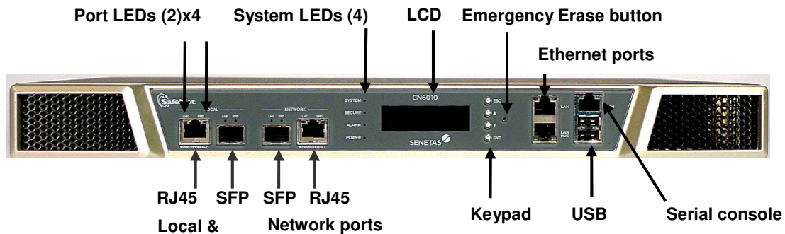
Figure 11 - Front View of the CN6010 [Y] Encryptor
