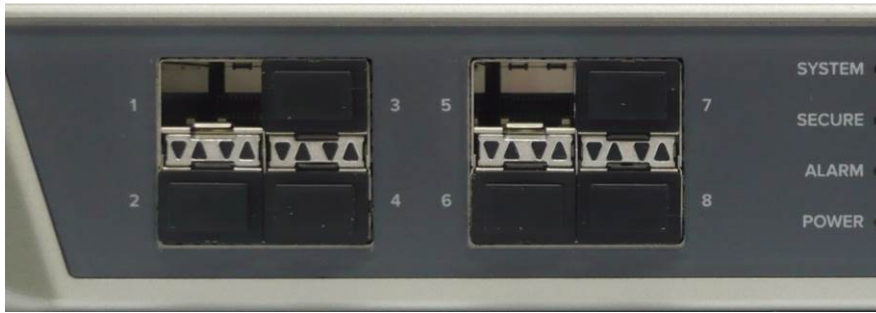
Figure 10 – A6140B Ethernet port close-up - SFPs not installed
