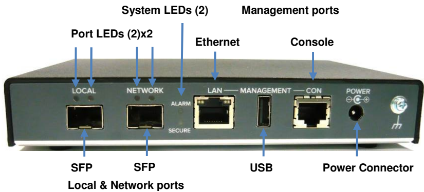
Figure 18 - Rear View of the CN4020 [O] and CN4020 [Y] Encryptors
