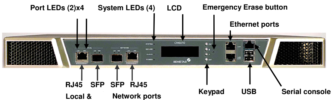
Figure 12 - Front View of the CN6010 [O] Encryptor
