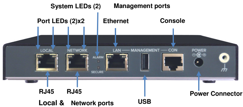
Figure 21 - Rear View of the CN4010 [O] and CN4010 [Y] Encryptors
