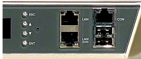
Figure 14 – CN6000 Series RJ45 Ethernet, Console and USB close-up
