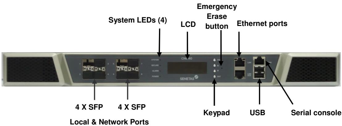
Figure 9 - Front View of the CN6140 [0] Encryptor
