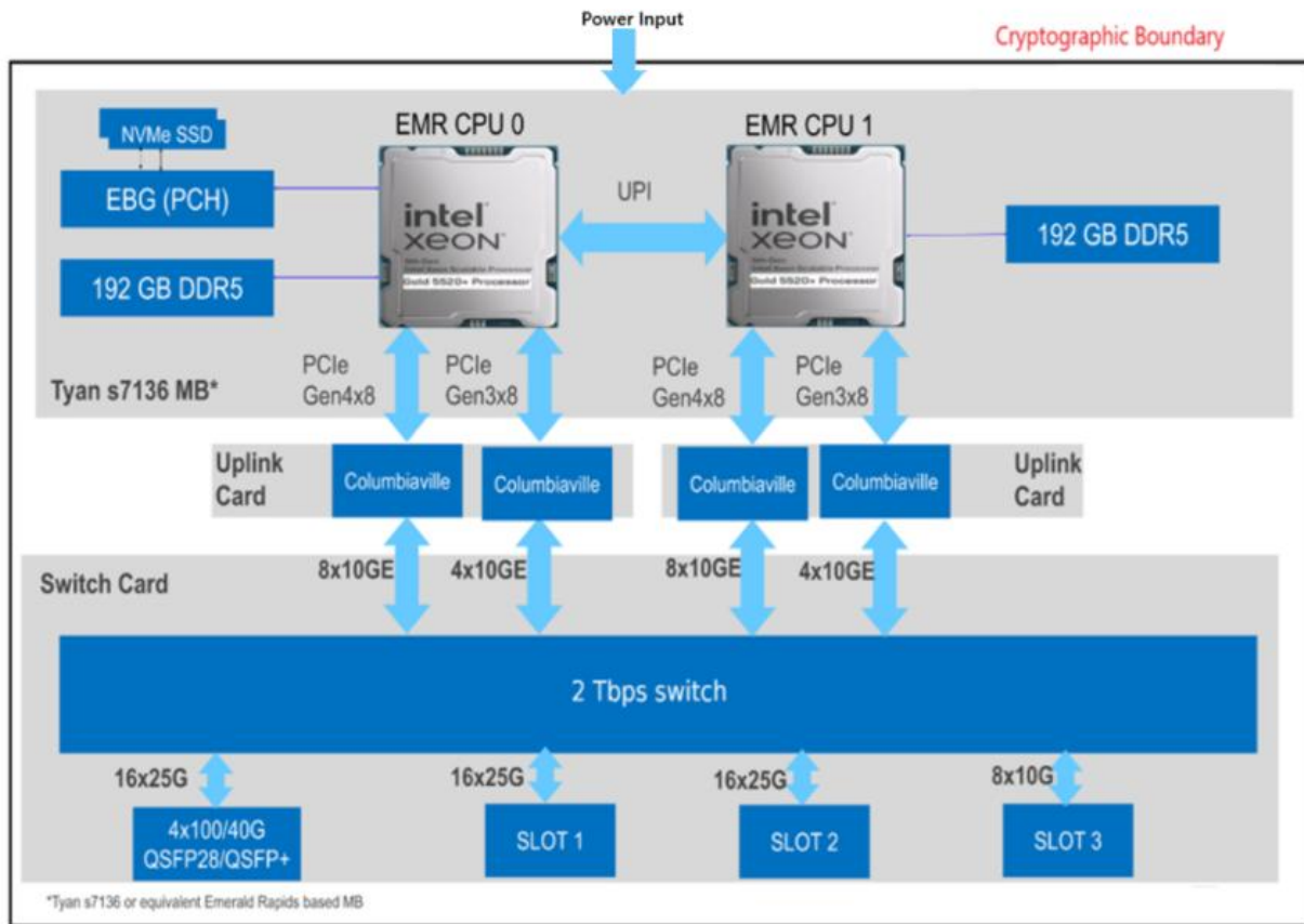
Figure 3: Block Diagram of the Trellix Intrusion Prevention System Sensor NS9600
