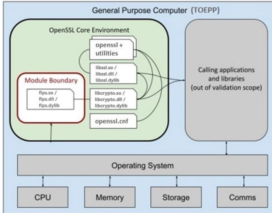
Figure 1: OVHCloud OKMS Provider based on the OpenSSL FIPS Provider Block Diagram
