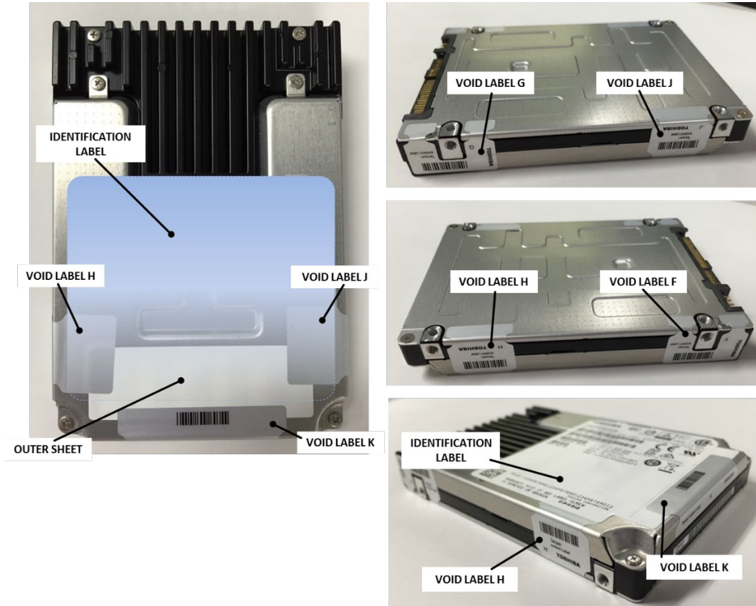
Figure 1 - Tamper-evident security seals
