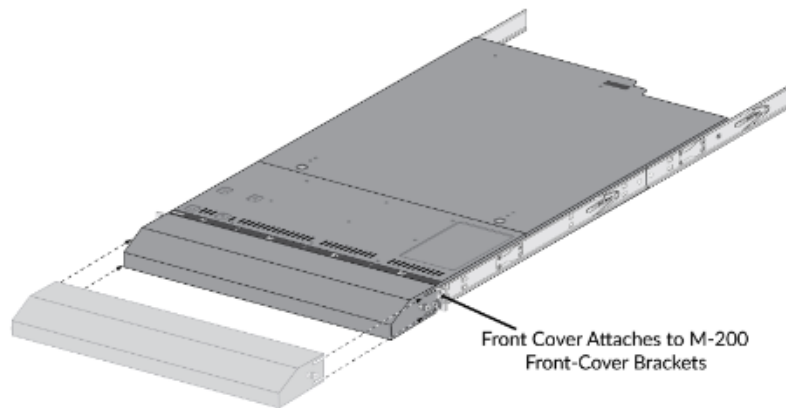
Figure 13 – M-200: Attach Physical Kit Front Cover
