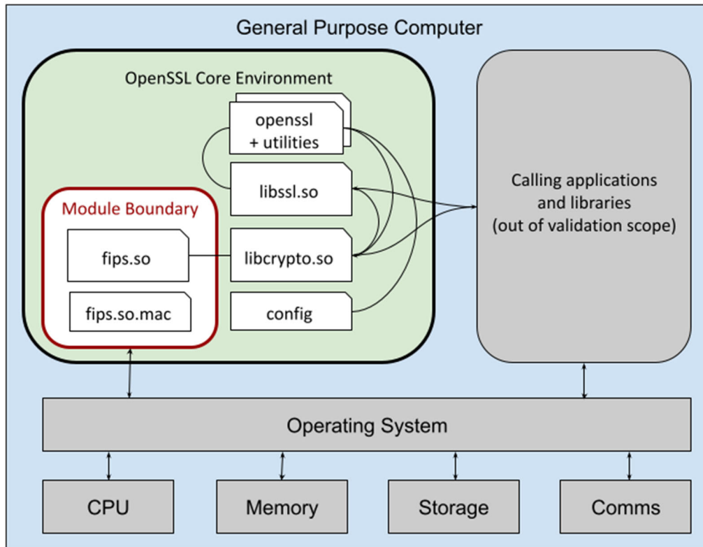
Figure 1: Block Diagram
