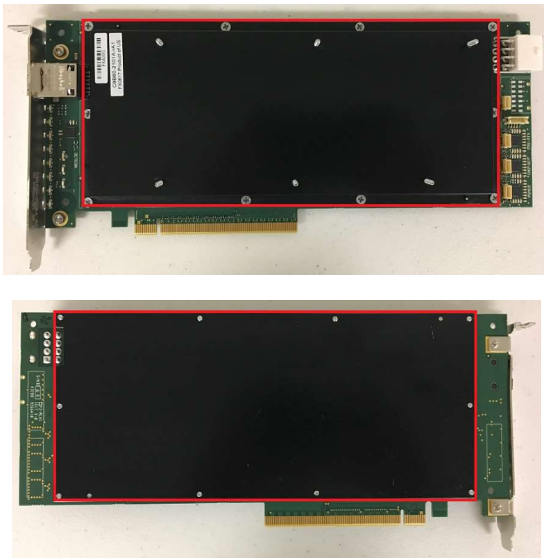
Figure 2: Front and back side of the Atalla Cryptographic Subsystem
