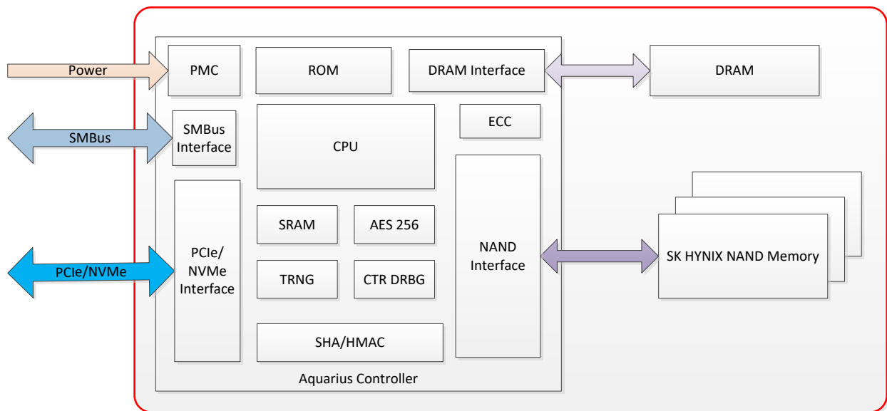
Figure 4: Module Block Diagram
