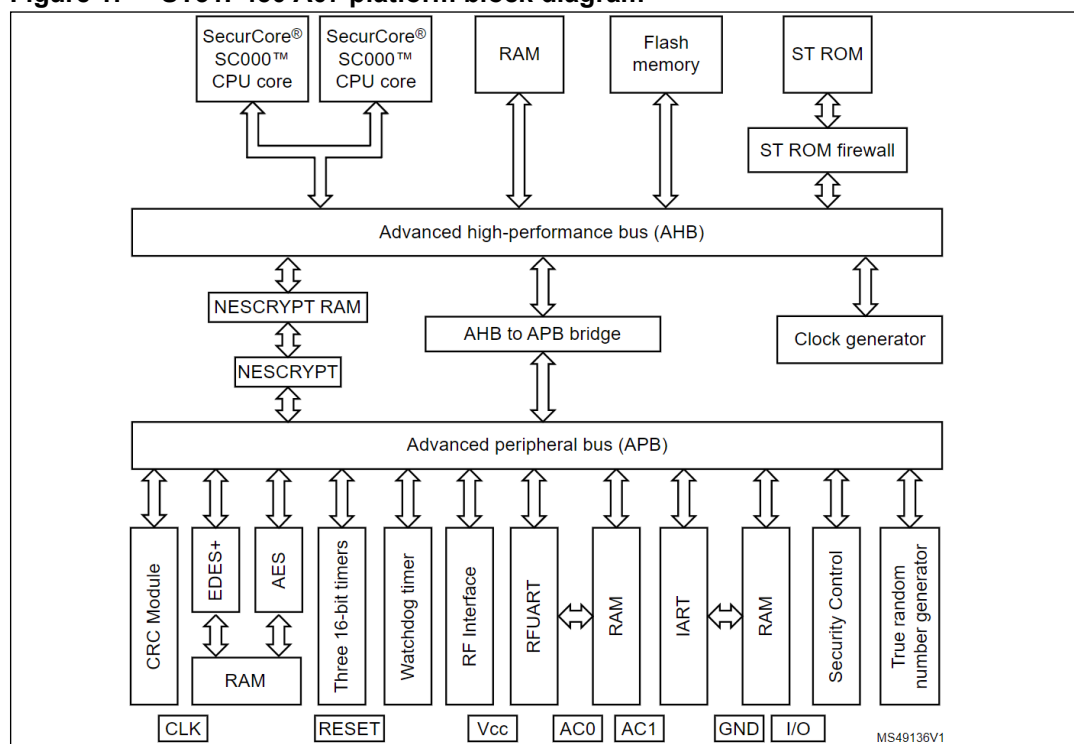
Figure 1. ST31P450 A07 platform block diagram
