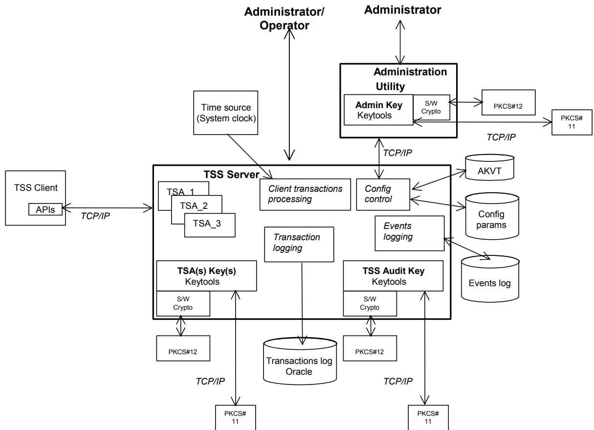
Figure 2.2 - Timestamp Server
