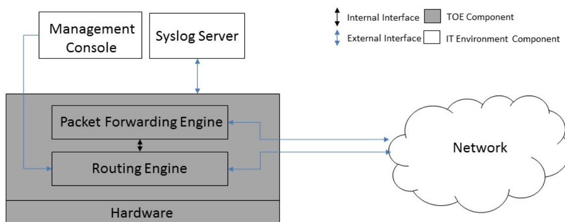
Figure 1 TOE Boundary for SRX345, SRX345-DUAL-AL and SRX380 models
