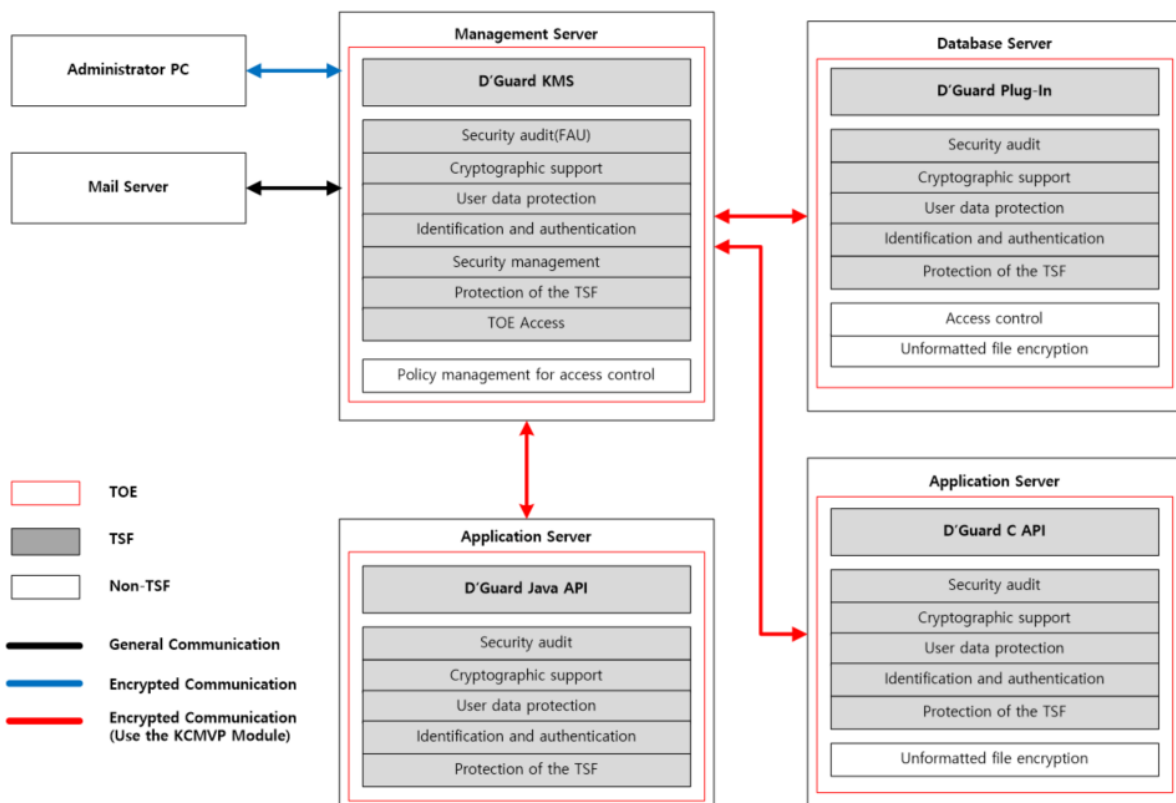
[Figure 5] Logical scope of the TOE
