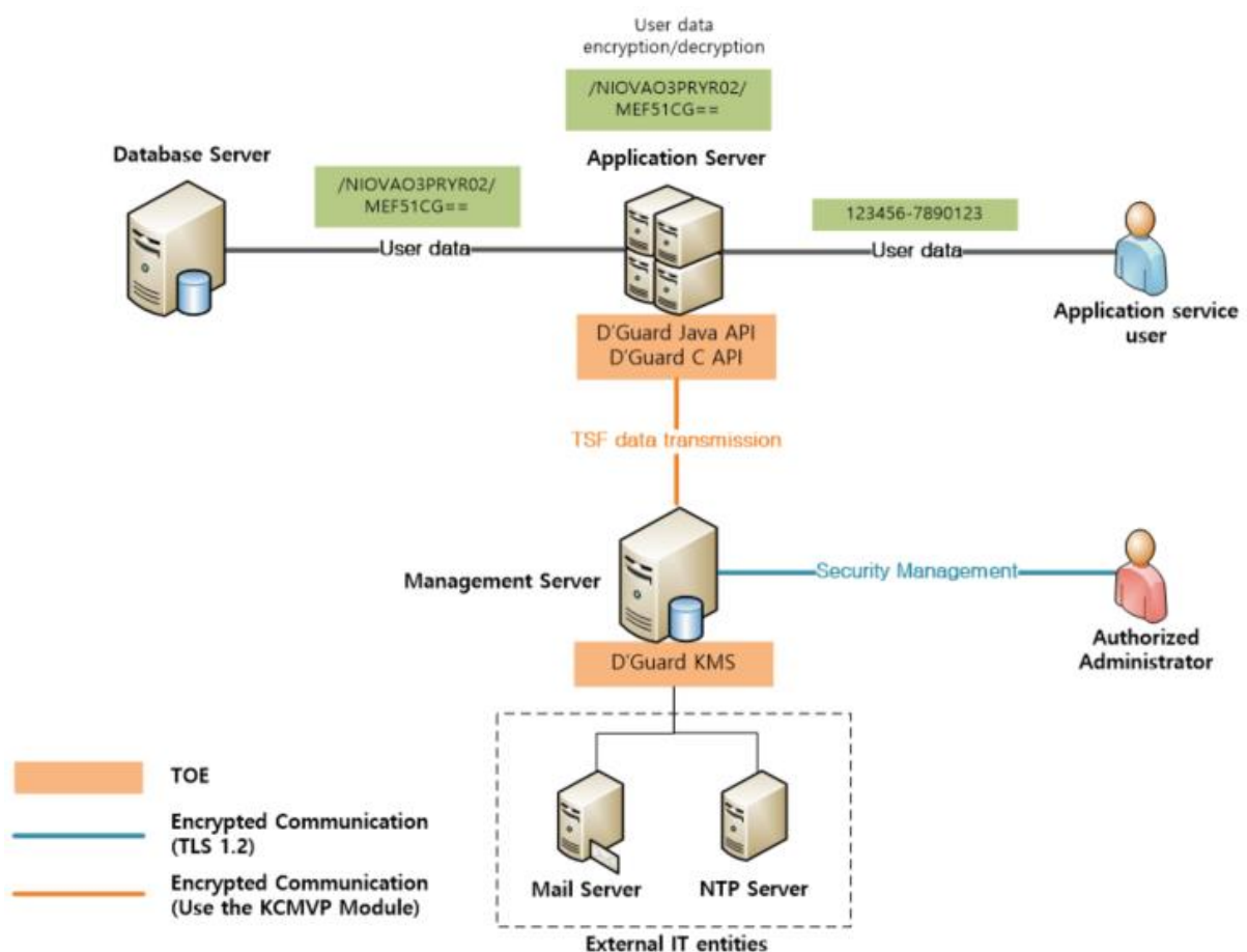
[Figure 2] API type operational environment
