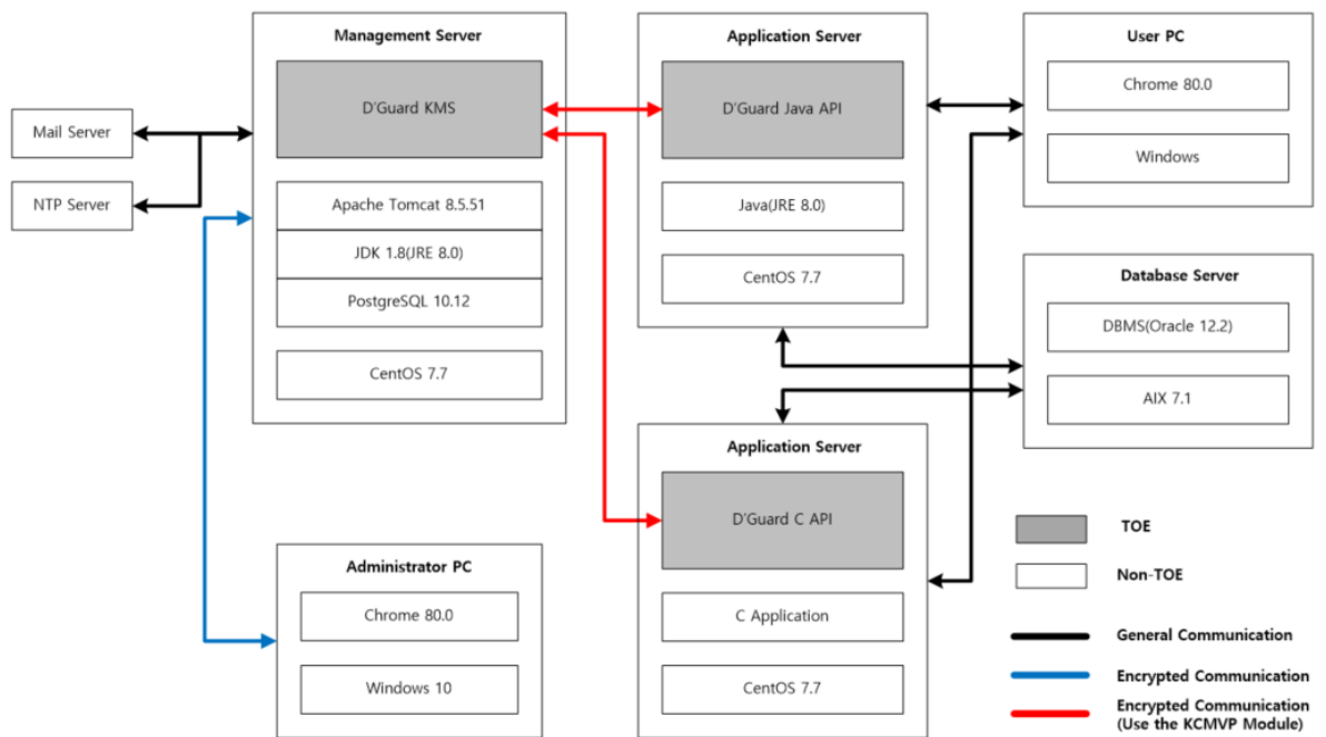
[Figure 4] Physical scope of the TOE (API type)
