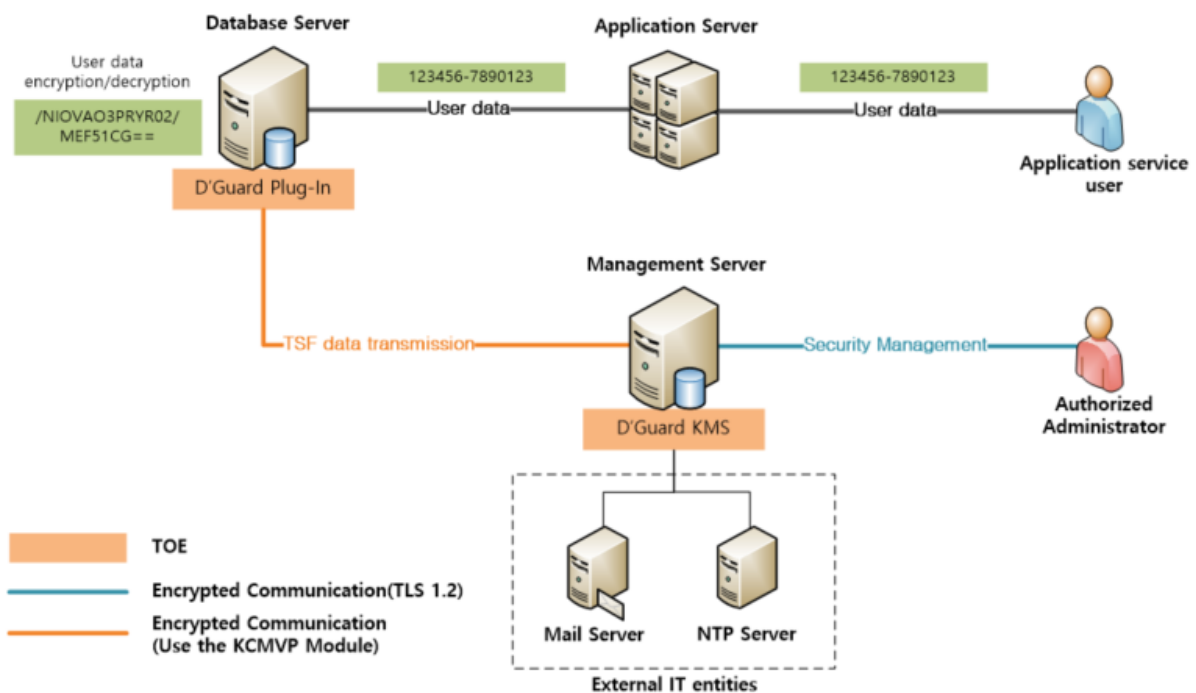
[Figure 1] Plug-In type operational environment
