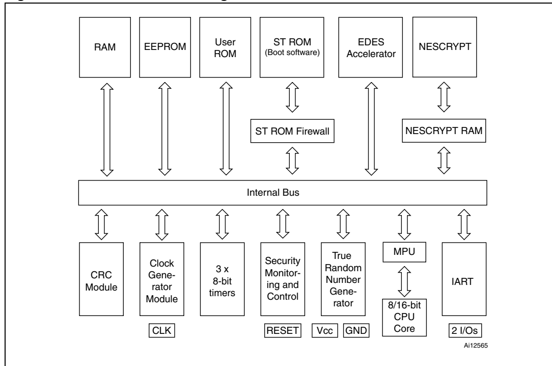
Figure 1. SA23YL18B block diagram
