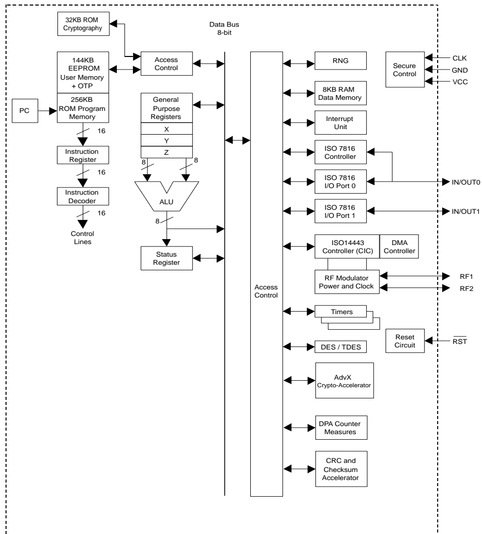
Figure 2-1 AT90SC256144RCFT / AT90SC25672RCFT Block Diagram
