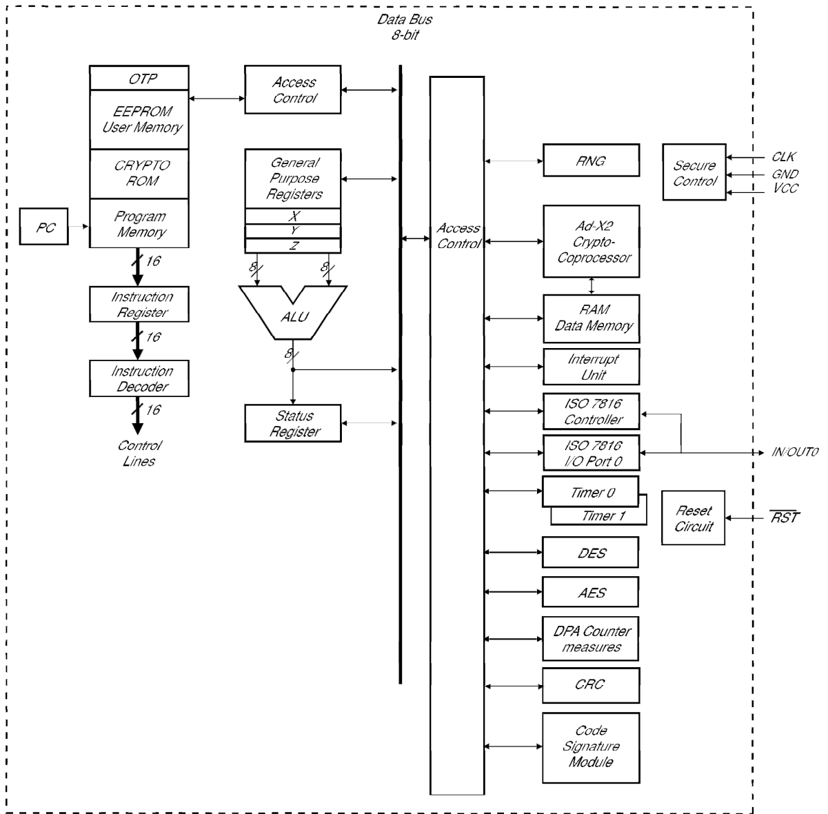
Figure 1: Block Diagram of the AT90SC28880RCV / AT90SC28848RCV TOE
