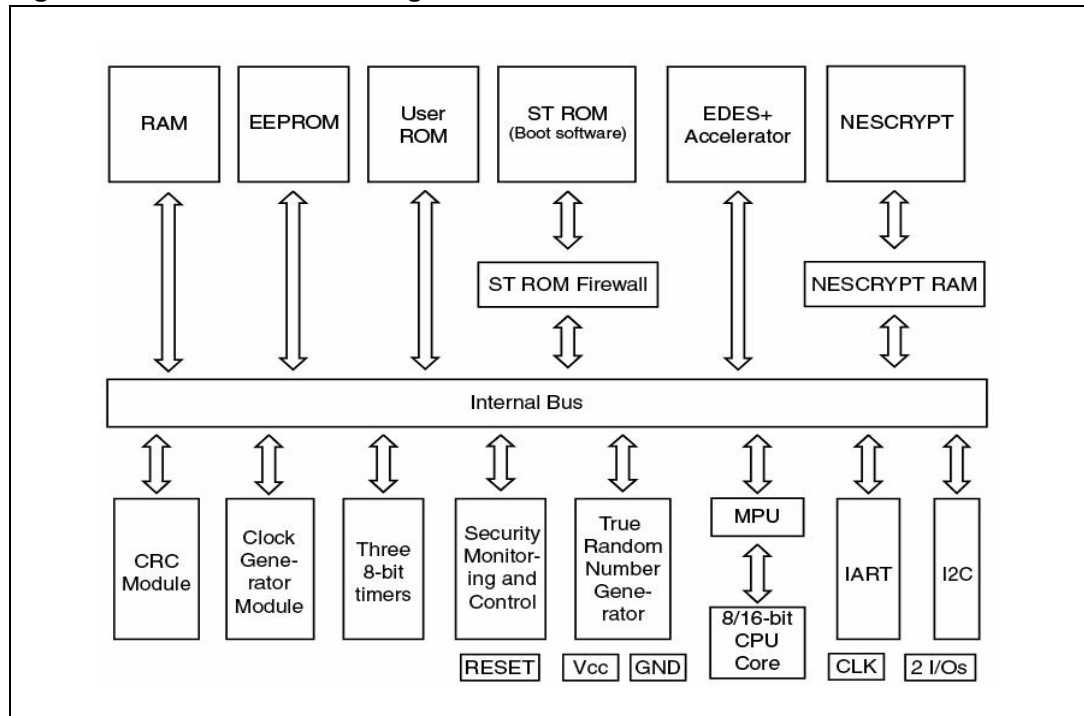
Figure 1. Sx23Zxxx block diagram
