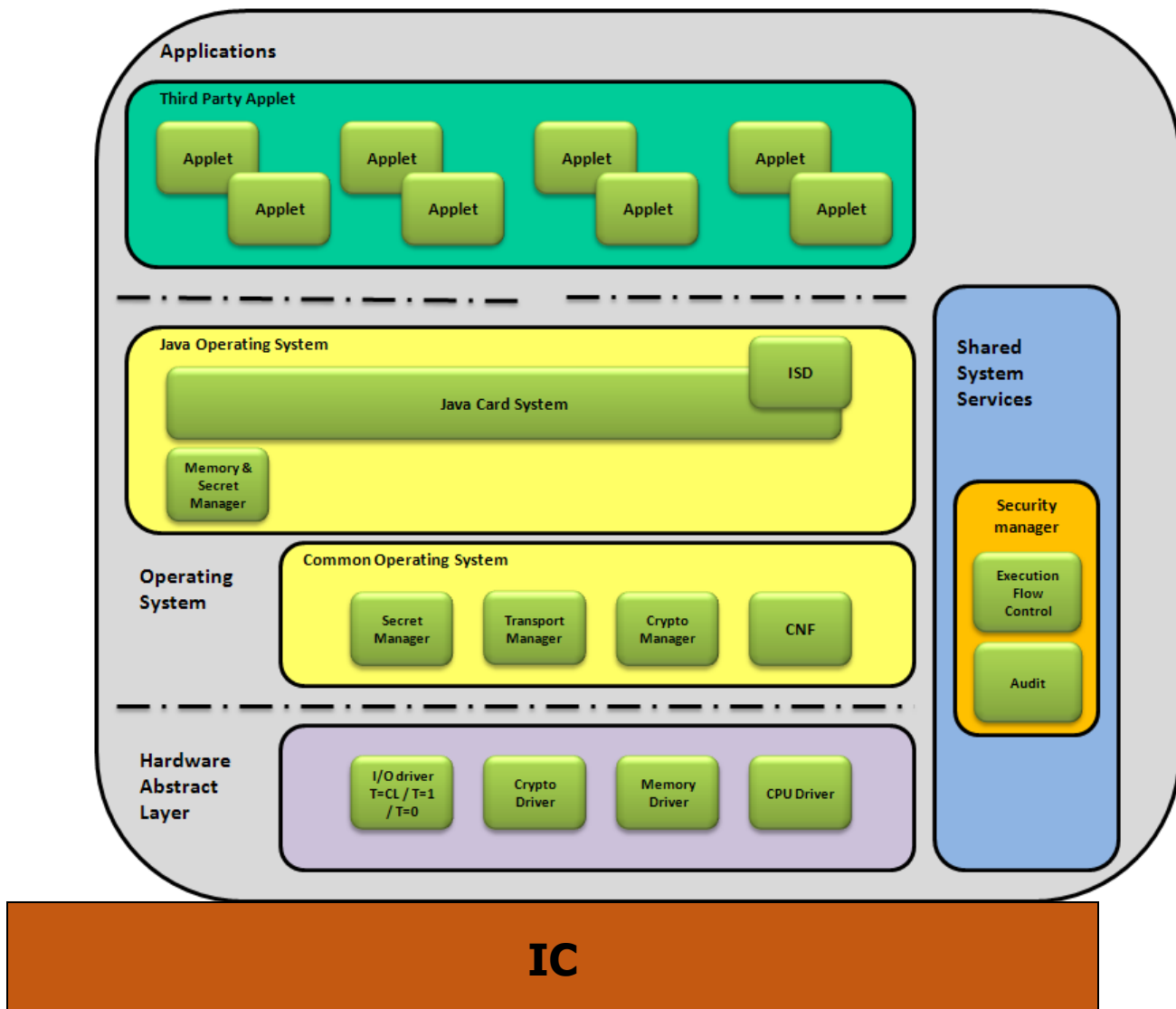
Figure 2 Product architecture
