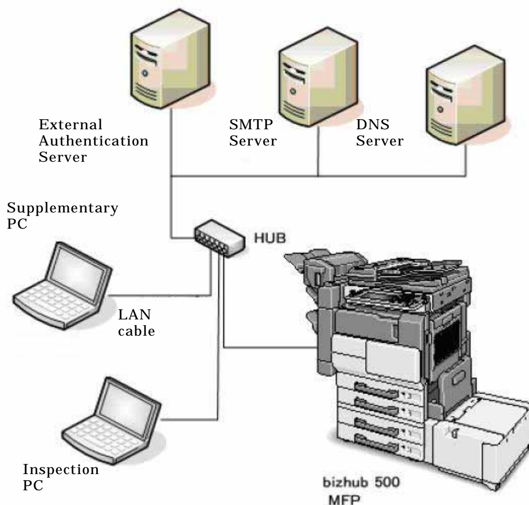
Figure2-2 Developer test (Intrusion test) configuration
