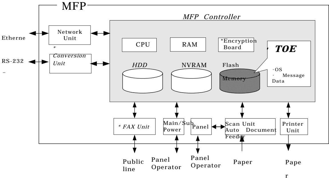
Figure 2-1 Configuration of Developer Testing
