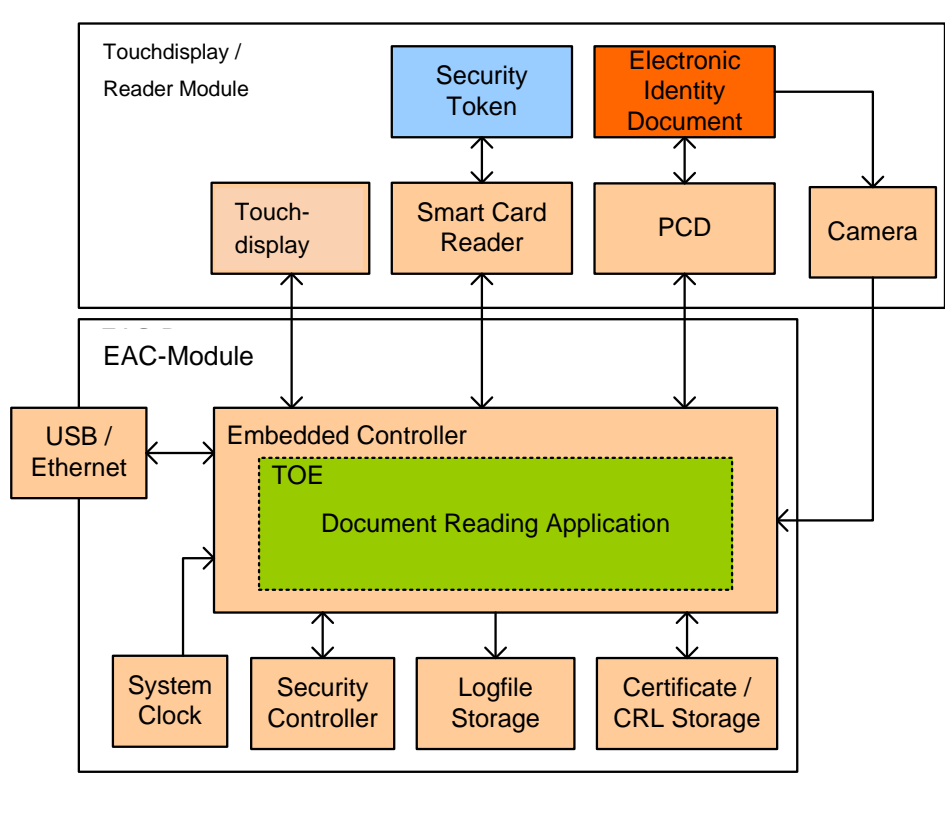
Figure 1: TOE demarcation
