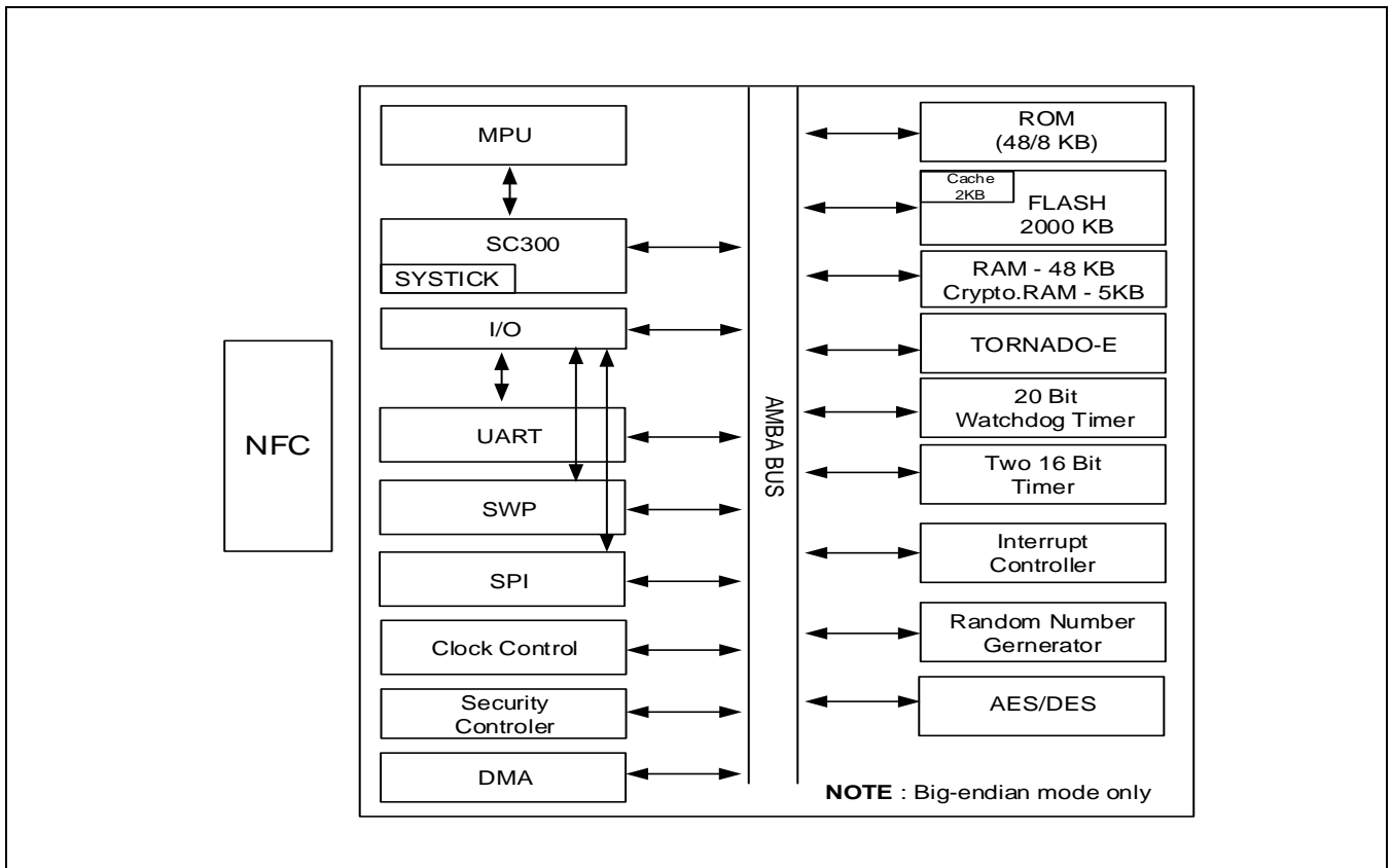
Figure 1 S3NSN4V Block Diagram
