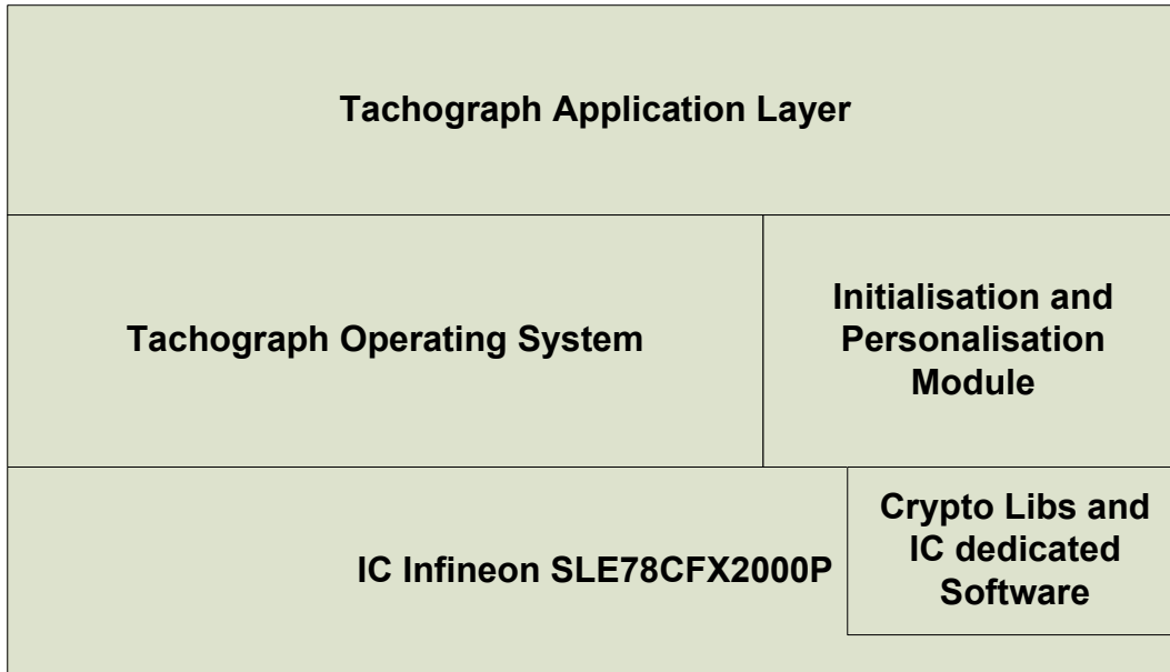
Figure 1: TOE Architecture
