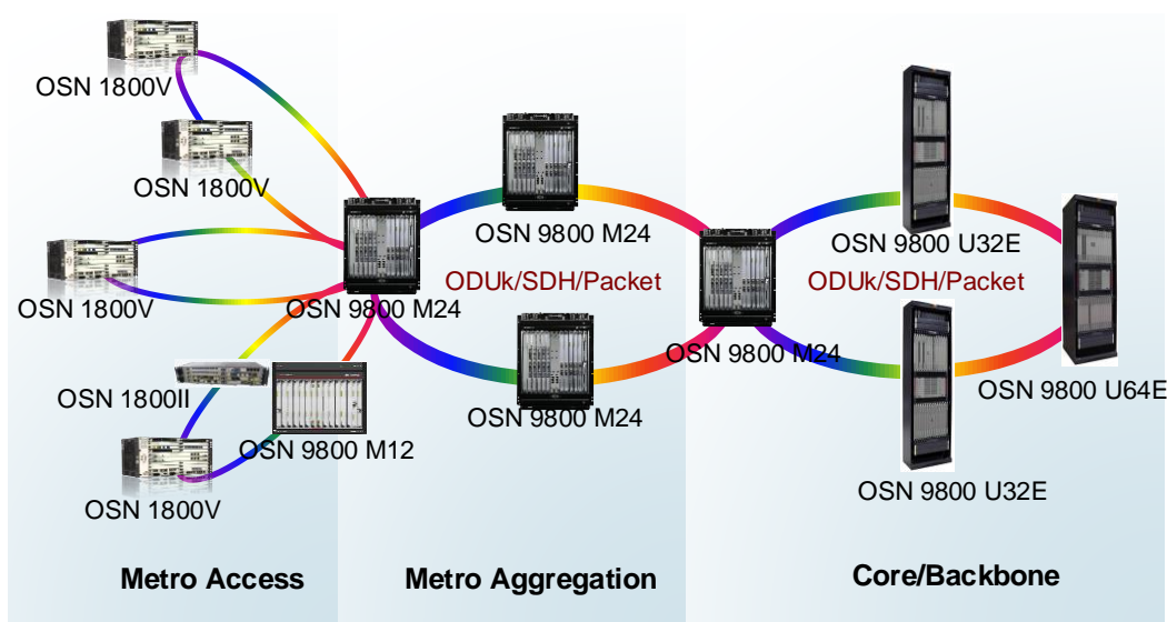
Figure 1-2 Position of the OSN Series on the entire network
