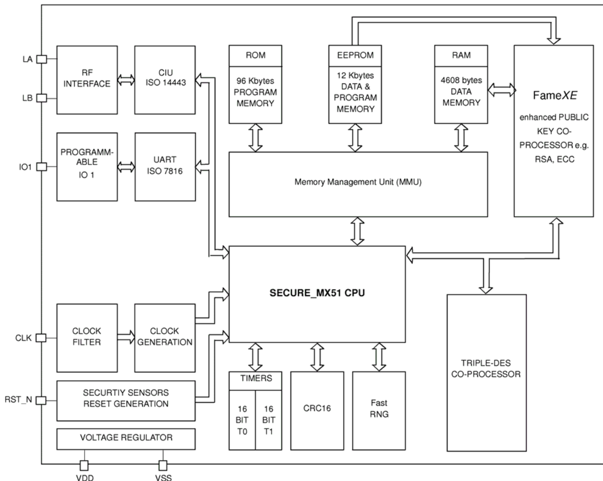
Figure 1: Block Diagram of the P5CD009V2B
