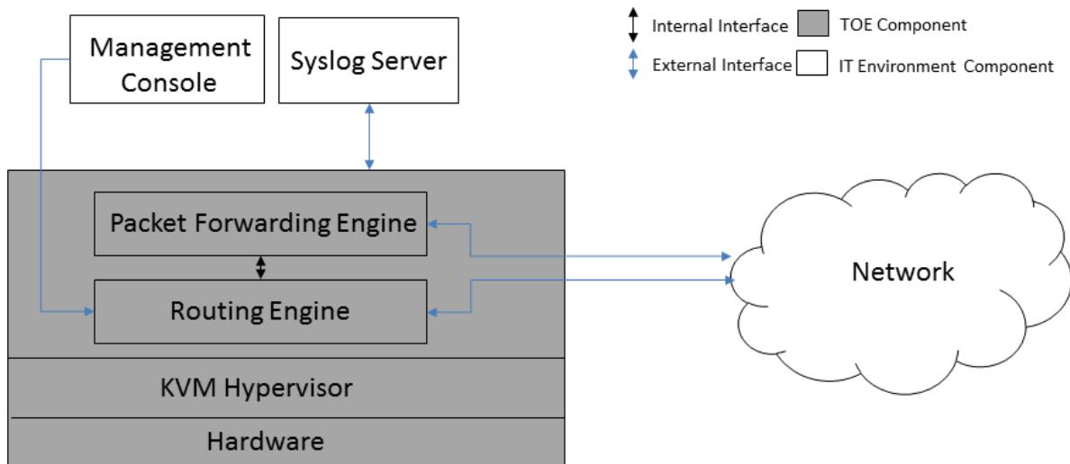
Figure 1 TOE Physical Boundary
