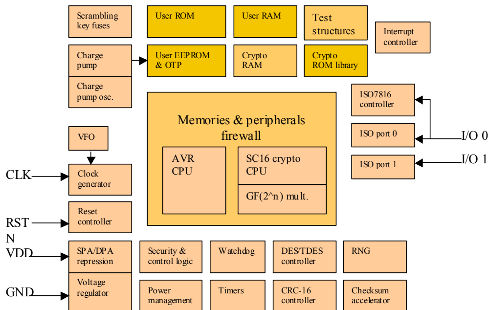
Figure 1 - micro-circuit ATMEL AT90SC9608RC
