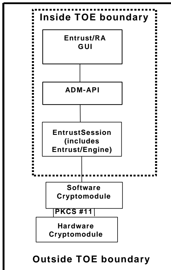
Figure 1: Entrust/RA architecture
