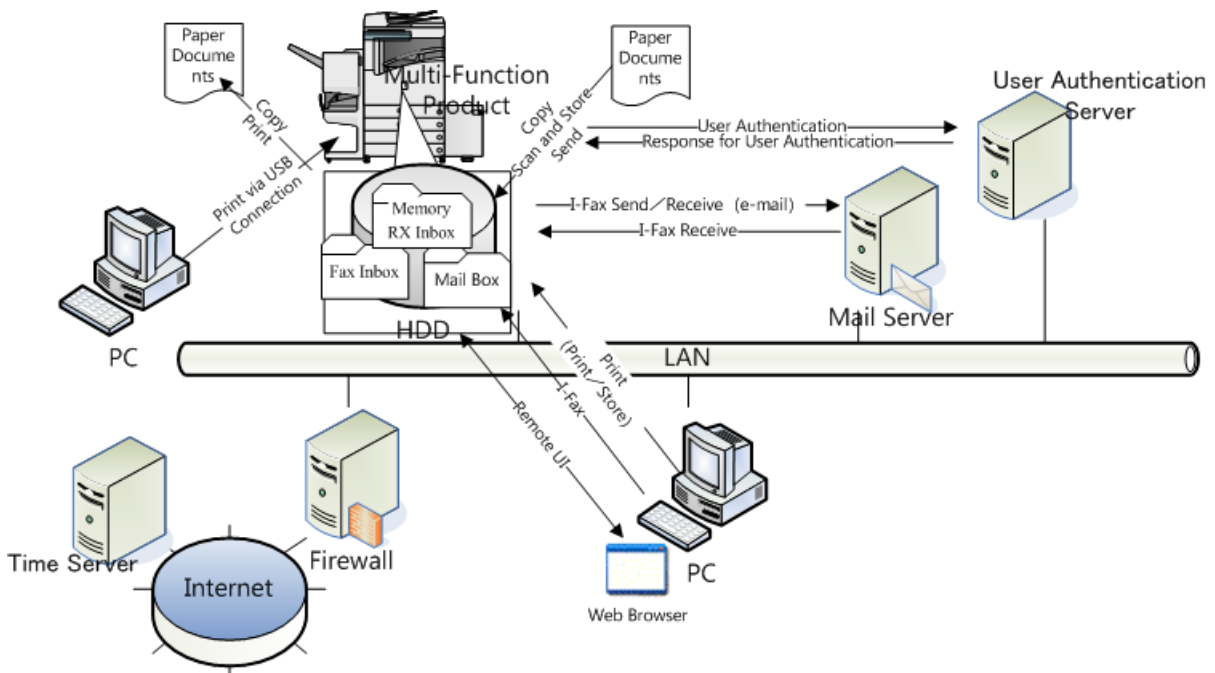
Figure 1 The assumed operational environment of the MFP < Canon imageRUNNER ADVANCE C5000 Series >
