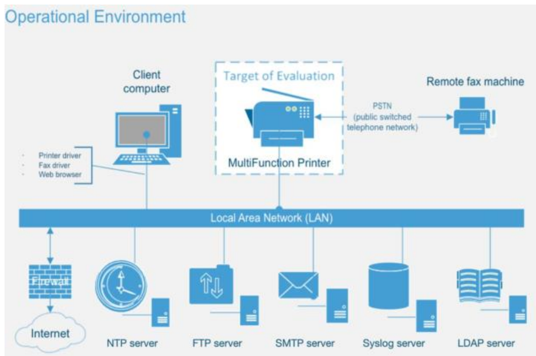
Figure 1: TOE Architecture
